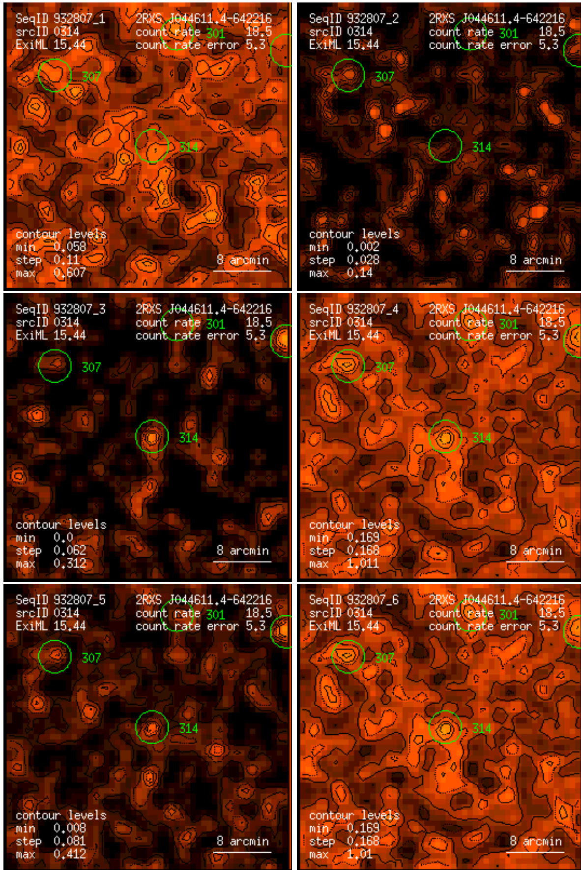
Figure 314: RASS 932807: detection 0314: band rate images, Gaussian filter: (1) PSPC channels 11 – 41, (2) 52 – 90, (3) 91 – 201, (4) 11 – 235, (5) 52 – 201, (6) 11 – 201. Broad band rates in counts/ks. Band rate contour levels in counts/ks/arcmin 2 .
