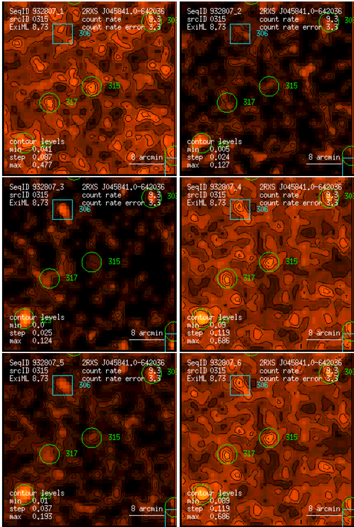
Figure 315: RASS 932807: detection 0315: band rate images, Gaussian filter: (1) PSPC channels 11 – 41, (2) 52 – 90, (3) 91 – 201, (4) 11 – 235, (5) 52 – 201, (6) 11 – 201. Broad band rates in counts/ks. Band rate contour levels in counts/ks/arcmin 2 .
