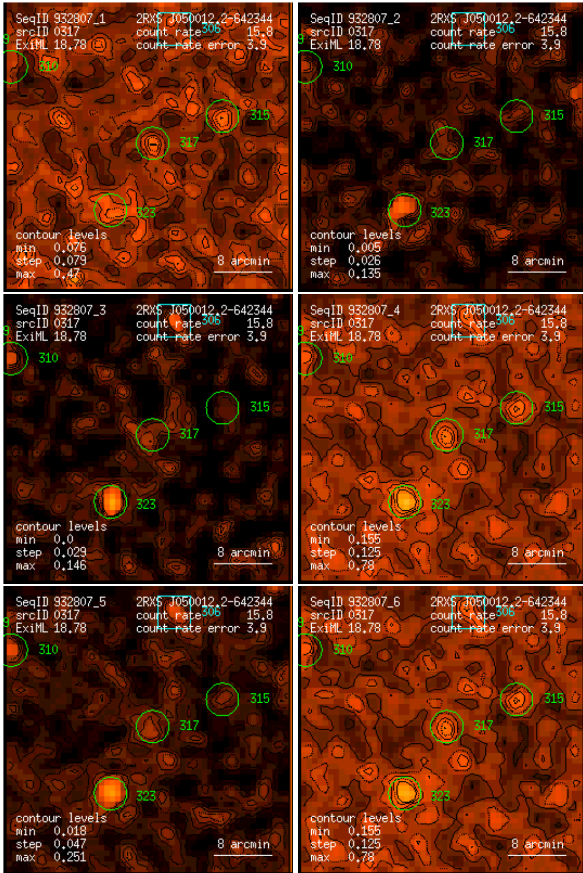
Figure 317: RASS 932807: detection 0317: band rate images, Gaussian filter: (1) PSPC channels 11 – 41, (2) 52 – 90, (3) 91 – 201, (4) 11 – 235, (5) 52 – 201, (6) 11 – 201. Broad band rates in counts/ks. Band rate contour levels in counts/ks/arcmin 2 .
