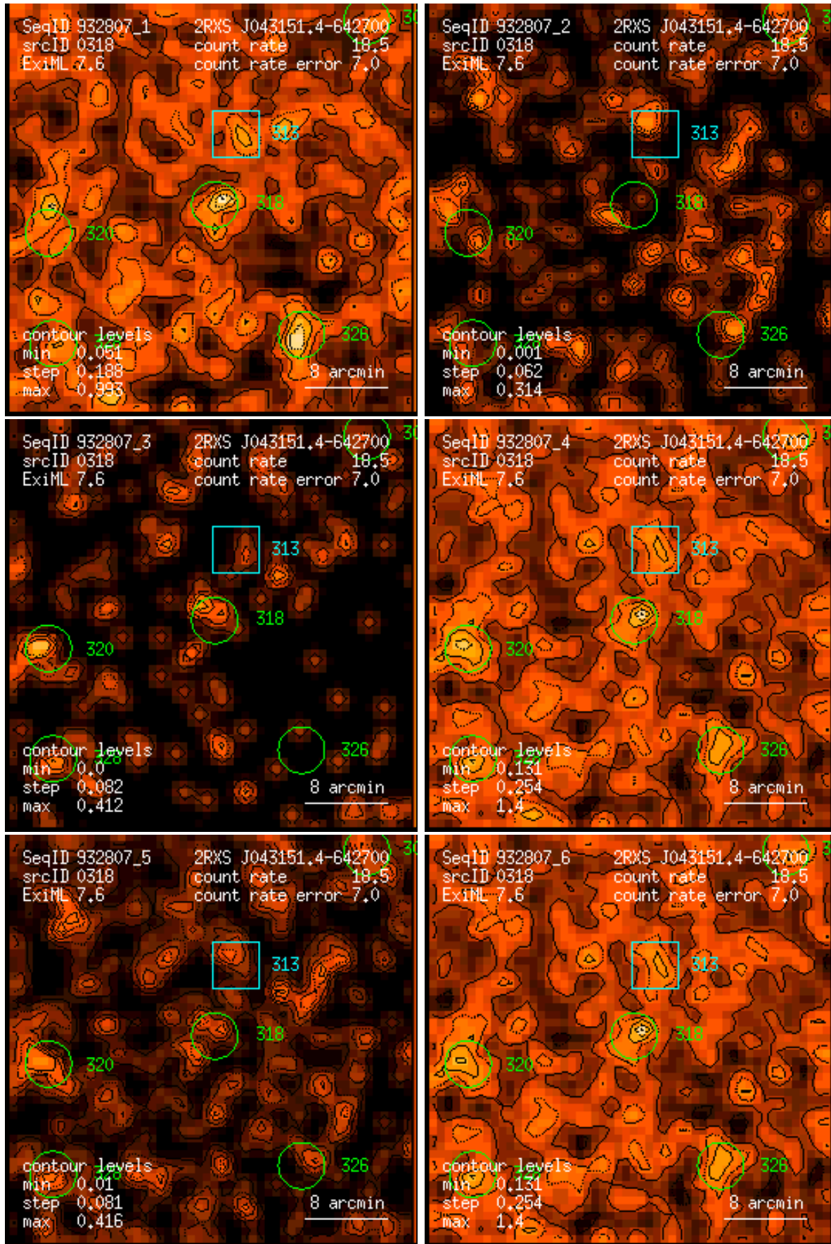
Figure 318: RASS 932807: detection 0318: band rate images, Gaussian filter: (1) PSPC channels 11 – 41, (2) 52 – 90, (3) 91 – 201, (4) 11 – 235, (5) 52 – 201, (6) 11 – 201. Broad band rates in counts/ks. Band rate contour levels in counts/ks/arcmin 2 .
