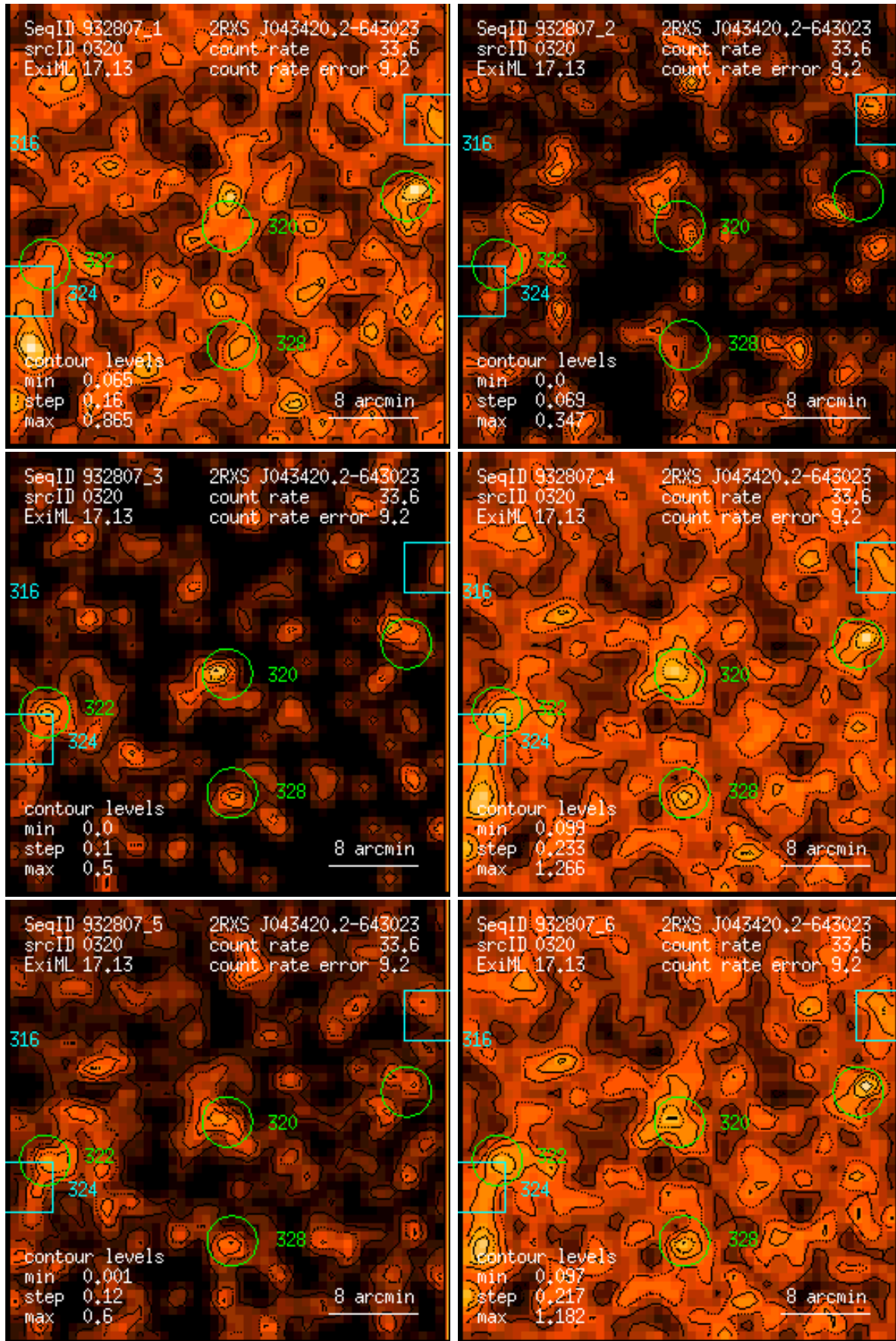
Figure 320: RASS 932807: detection 0320: band rate images, Gaussian filter: (1) PSPC channels 11 – 41, (2) 52 – 90, (3) 91 – 201, (4) 11 – 235, (5) 52 – 201, (6) 11 – 201. Broad band rates in counts/ks. Band rate contour levels in counts/ks/arcmin 2 .
