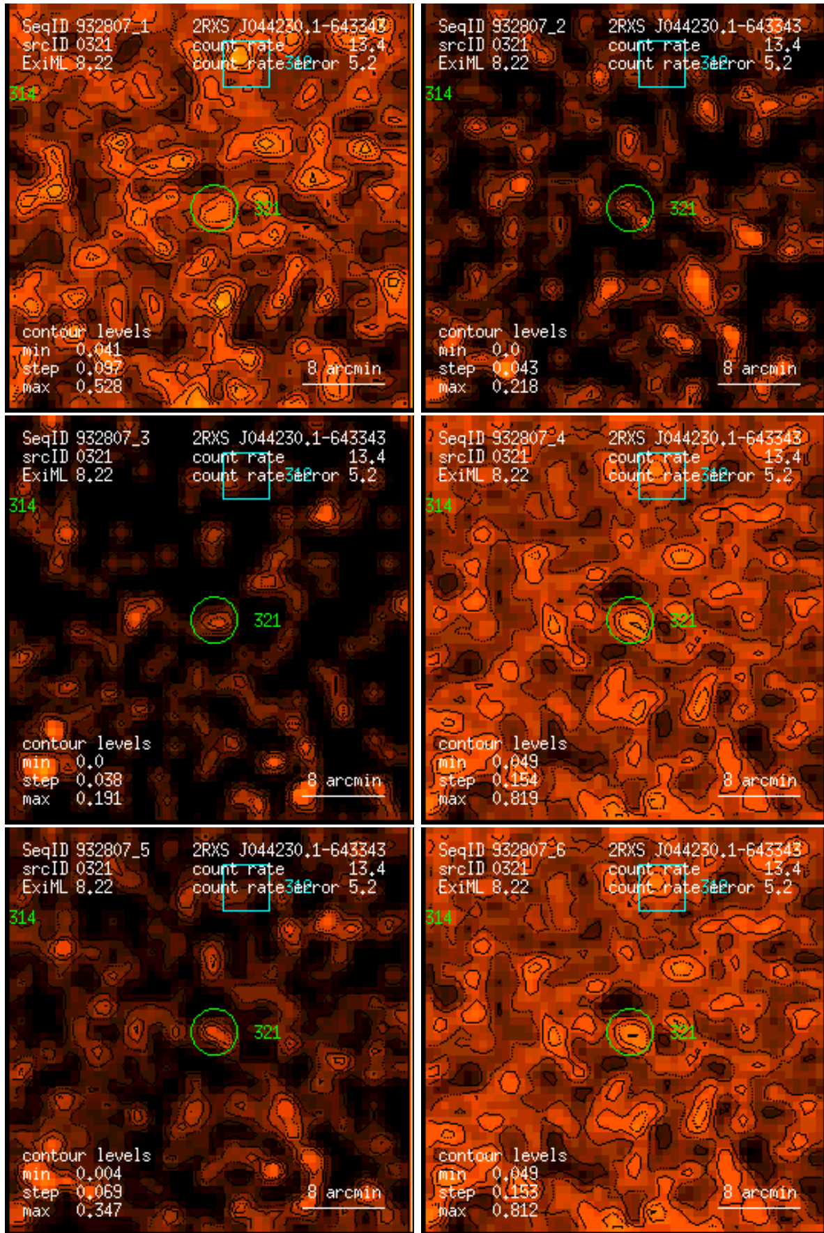
Figure 321: RASS 932807: detection 0321: band rate images, Gaussian filter: (1) PSPC channels 11 – 41, (2) 52 – 90, (3) 91 – 201, (4) 11 – 235, (5) 52 – 201, (6) 11 – 201. Broad band rates in counts/ks. Band rate contour levels in counts/ks/arcmin 2 .
