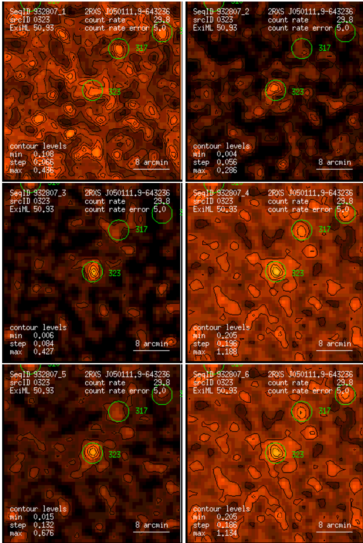
Figure 323: RASS 932807: detection 0323: band rate images, Gaussian filter: (1) PSPC channels 11 – 41, (2) 52 – 90, (3) 91 – 201, (4) 11 – 235, (5) 52 – 201, (6) 11 – 201. Broad band rates in counts/ks. Band rate contour levels in counts/ks/arcmin 2 .
