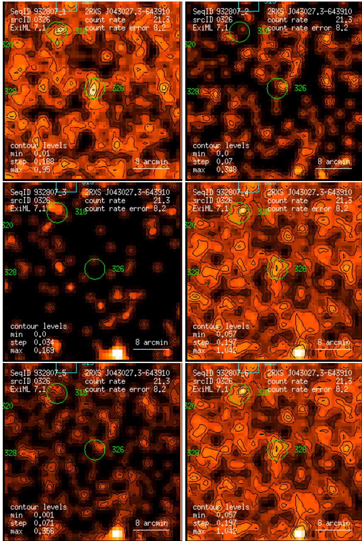
Figure 326: RASS 932807: detection 0326: band rate images, Gaussian filter: (1) PSPC channels 11 – 41, (2) 52 – 90, (3) 91 – 201, (4) 11 – 235, (5) 52 – 201, (6) 11 – 201. Broad band rates in counts/ks. Band rate contour levels in counts/ks/arcmin 2 .
