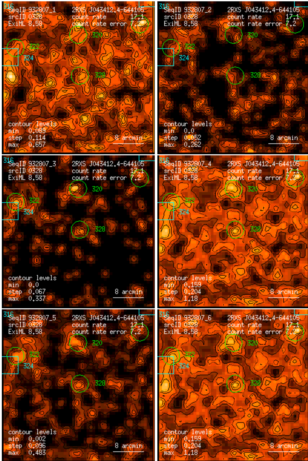
Figure 328: RASS 932807: detection 0328: band rate images, Gaussian filter: (1) PSPC channels 11 – 41, (2) 52 – 90, (3) 91 – 201, (4) 11 – 235, (5) 52 – 201, (6) 11 – 201. Broad band rates in counts/ks. Band rate contour levels in counts/ks/arcmin 2 .
