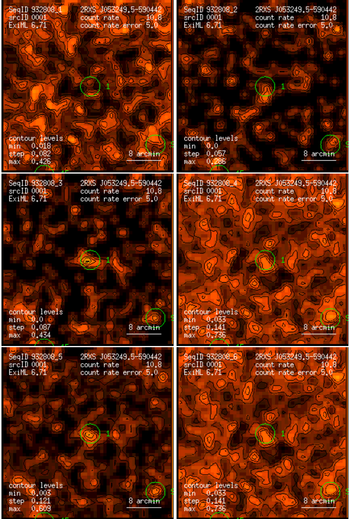
Figure 1: RASS 932808: detection 0001: band rate images, Gaussian filter: (1) PSPC channels 11 – 41, (2) 52 – 90, (3) 91 – 201, (4) 11 – 235, (5) 52 – 201, (6) 11 – 201. Broad band rates in counts/ks. Band rate contour levels in counts/ks/arcmin 2 .
