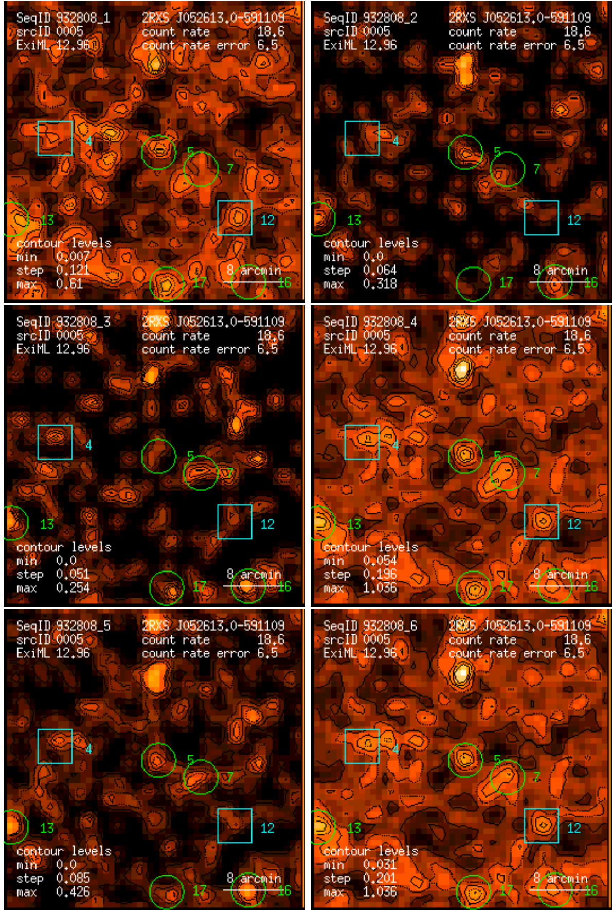
Figure 5: RASS 932808: detection 0005: band rate images, Gaussian filter: (1) PSPC channels 11 – 41, (2) 52 – 90, (3) 91 – 201, (4) 11 – 235, (5) 52 – 201, (6) 11 – 201. Broad band rates in counts/ks. Band rate contour levels in counts/ks/arcmin 2 .
