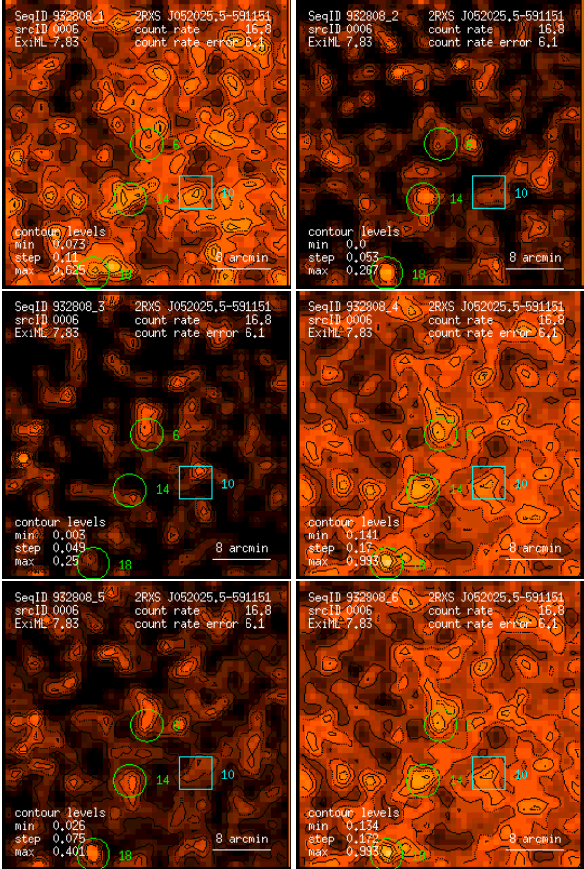
Figure 6: RASS 932808: detection 0006: band rate images, Gaussian filter: (1) PSPC channels 11 – 41, (2) 52 – 90, (3) 91 – 201, (4) 11 – 235, (5) 52 – 201, (6) 11 – 201. Broad band rates in counts/ks. Band rate contour levels in counts/ks/arcmin 2 .
