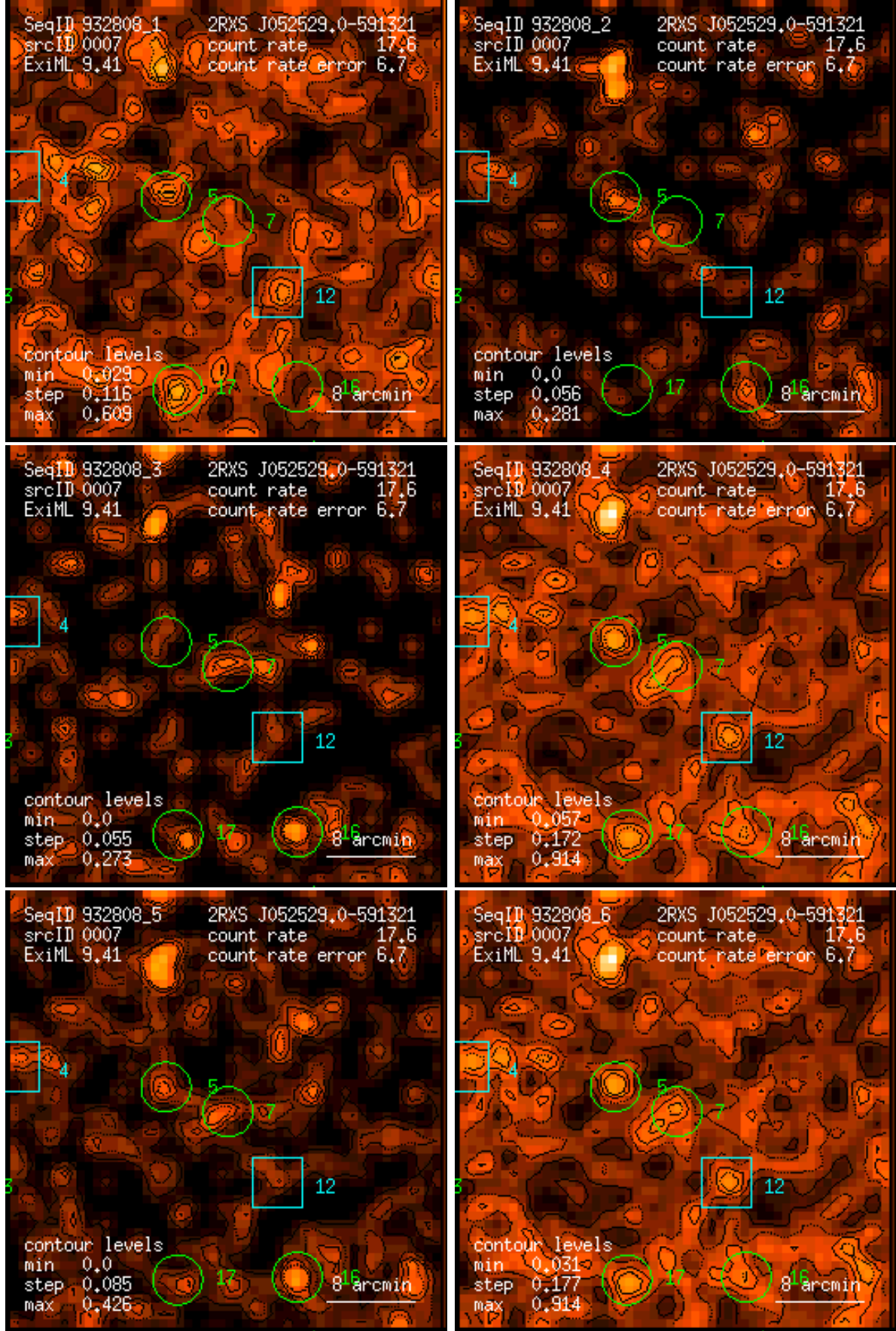
Figure 7: RASS 932808: detection 0007: band rate images, Gaussian filter: (1) PSPC channels 11 – 41, (2) 52 – 90, (3) 91 – 201, (4) 11 – 235, (5) 52 – 201, (6) 11 – 201. Broad band rates in counts/ks. Band rate contour levels in counts/ks/arcmin 2 .
