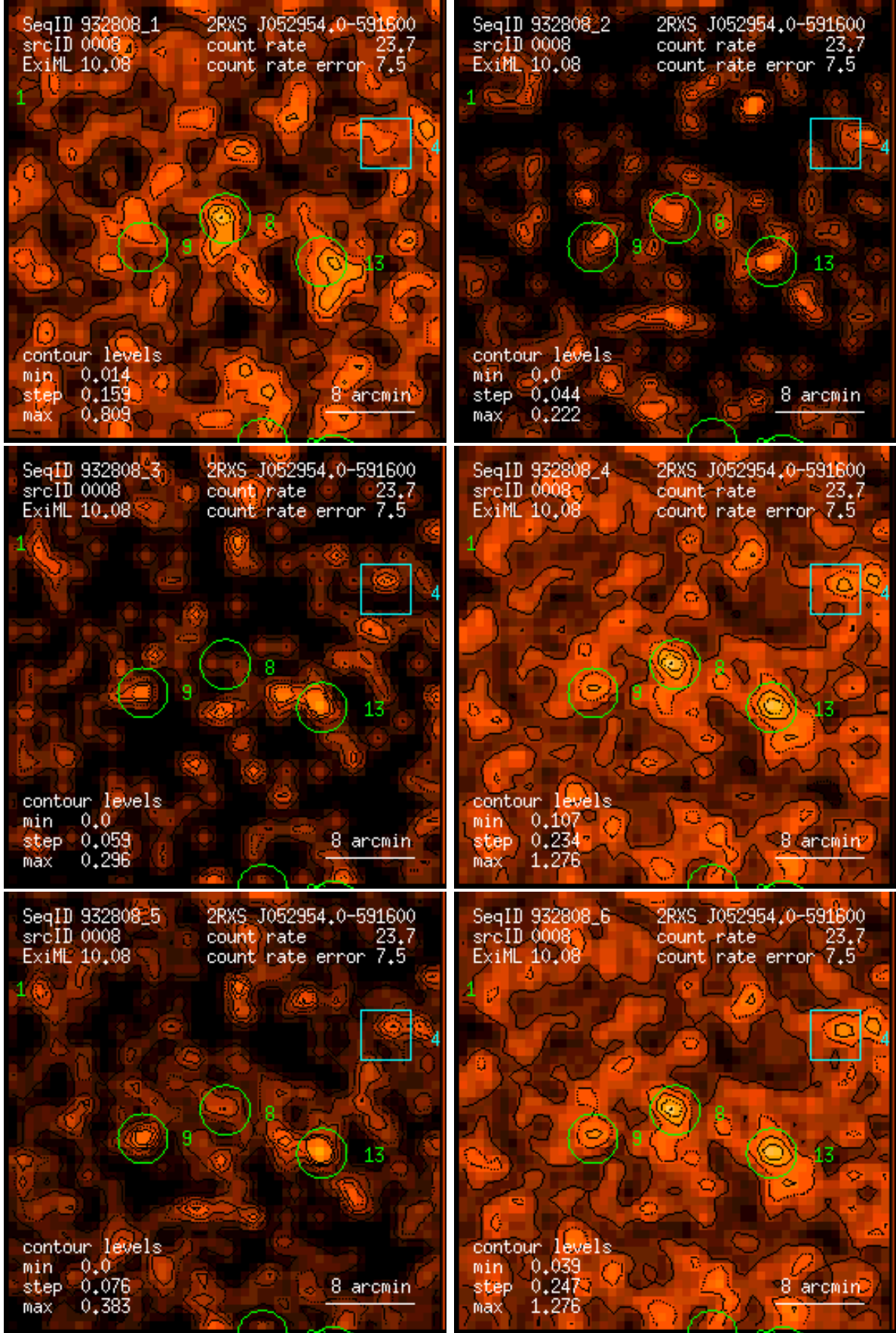
Figure 8: RASS 932808: detection 0008: band rate images, Gaussian filter: (1) PSPC channels 11 – 41, (2) 52 – 90, (3) 91 – 201, (4) 11 – 235, (5) 52 – 201, (6) 11 – 201. Broad band rates in counts/ks. Band rate contour levels in counts/ks/arcmin 2 .
