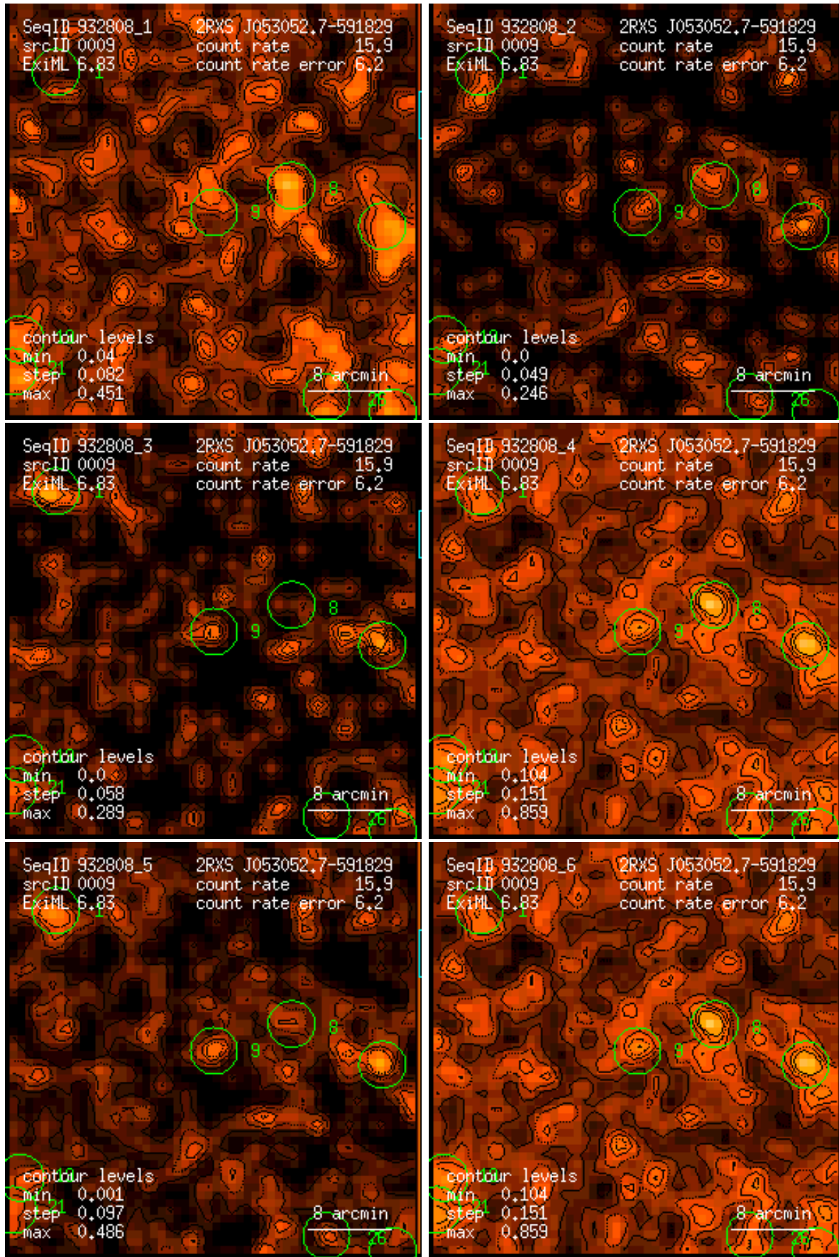
Figure 9: RASS 932808: detection 0009: band rate images, Gaussian filter: (1) PSPC channels 11 – 41, (2) 52 – 90, (3) 91 – 201, (4) 11 – 235, (5) 52 – 201, (6) 11 – 201. Broad band rates in counts/ks. Band rate contour levels in counts/ks/arcmin 2 .
