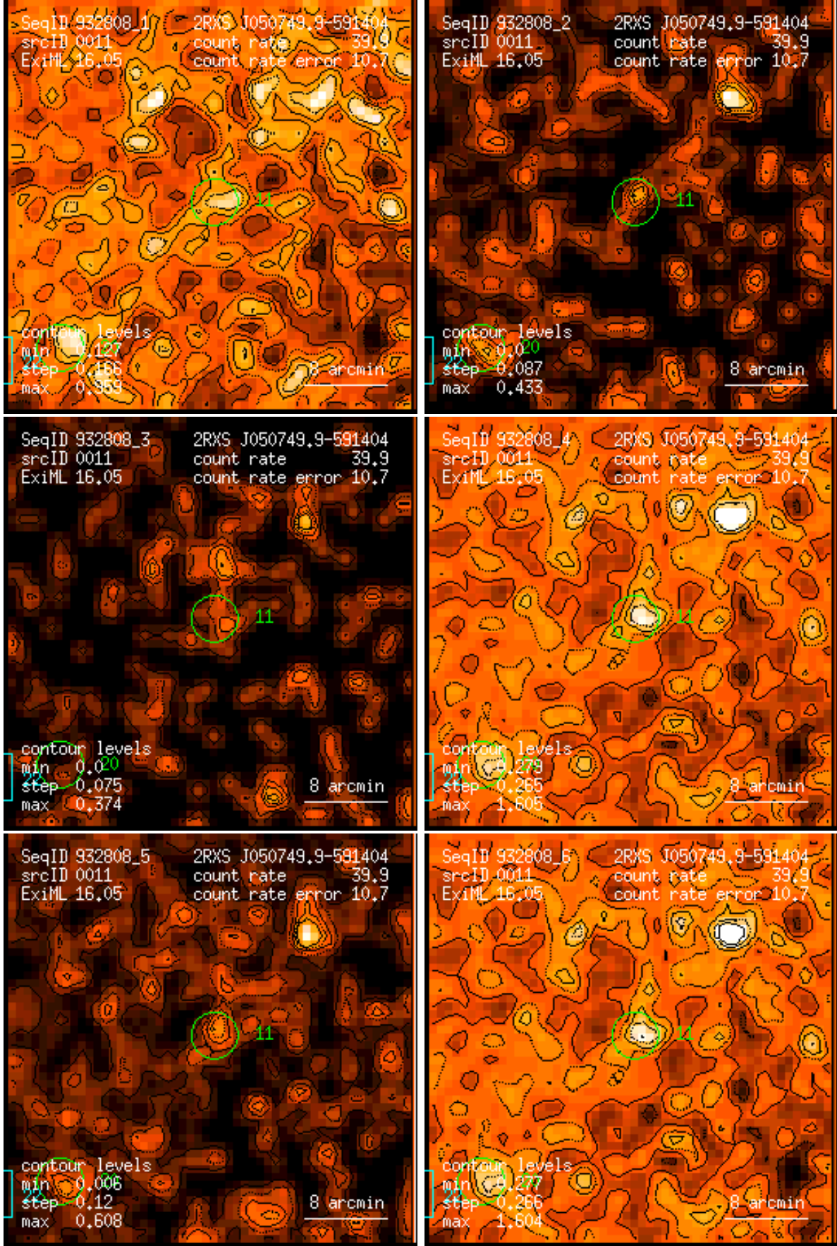
Figure 11: RASS 932808: detection 0011: band rate images, Gaussian filter: (1) PSPC channels 11 – 41, (2) 52 – 90, (3) 91 – 201, (4) 11 – 235, (5) 52 – 201, (6) 11 – 201. Broad band rates in counts/ks. Band rate contour levels in counts/ks/arcmin 2 .
