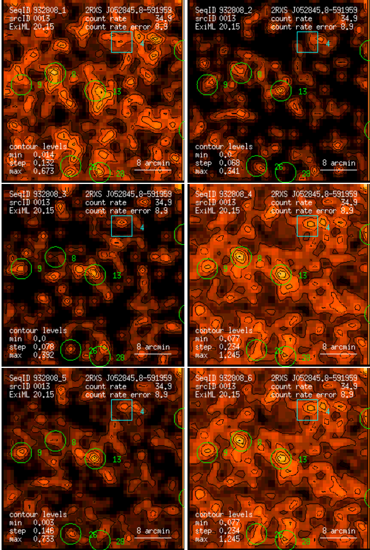
Figure 13: RASS 932808: detection 0013: band rate images, Gaussian filter: (1) PSPC channels 11 – 41, (2) 52 – 90, (3) 91 – 201, (4) 11 – 235, (5) 52 – 201, (6) 11 – 201. Broad band rates in counts/ks. Band rate contour levels in counts/ks/arcmin 2 .
