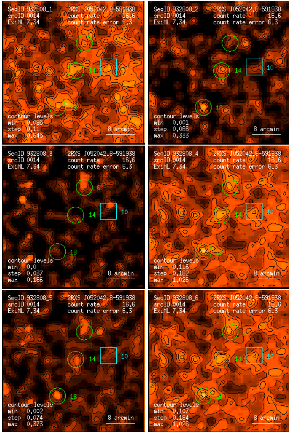
Figure 14: RASS 932808: detection 0014: band rate images, Gaussian filter: (1) PSPC channels 11 – 41, (2) 52 – 90, (3) 91 – 201, (4) 11 – 235, (5) 52 – 201, (6) 11 – 201. Broad band rates in counts/ks. Band rate contour levels in counts/ks/arcmin 2 .
