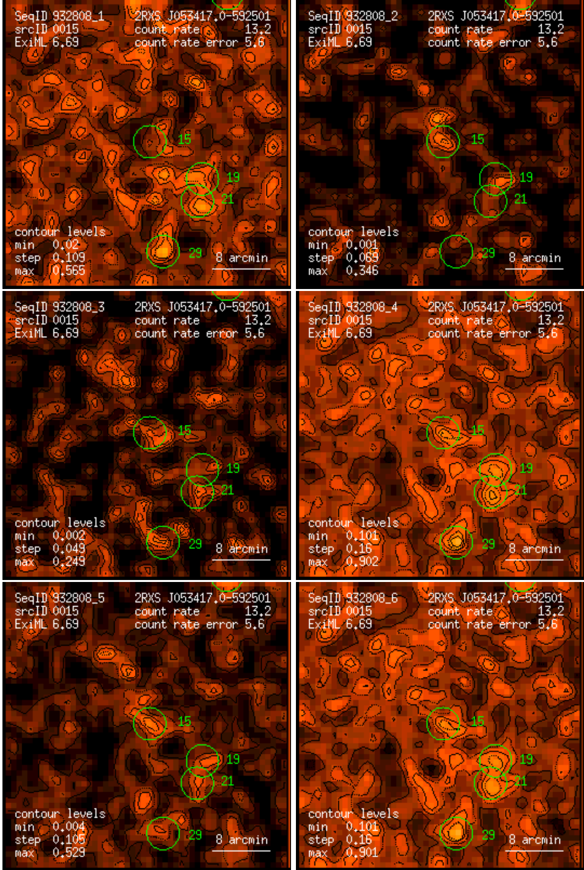
Figure 15: RASS 932808: detection 0015: band rate images, Gaussian filter: (1) PSPC channels 11 – 41, (2) 52 – 90, (3) 91 – 201, (4) 11 – 235, (5) 52 – 201, (6) 11 – 201. Broad band rates in counts/ks. Band rate contour levels in counts/ks/arcmin 2 .
