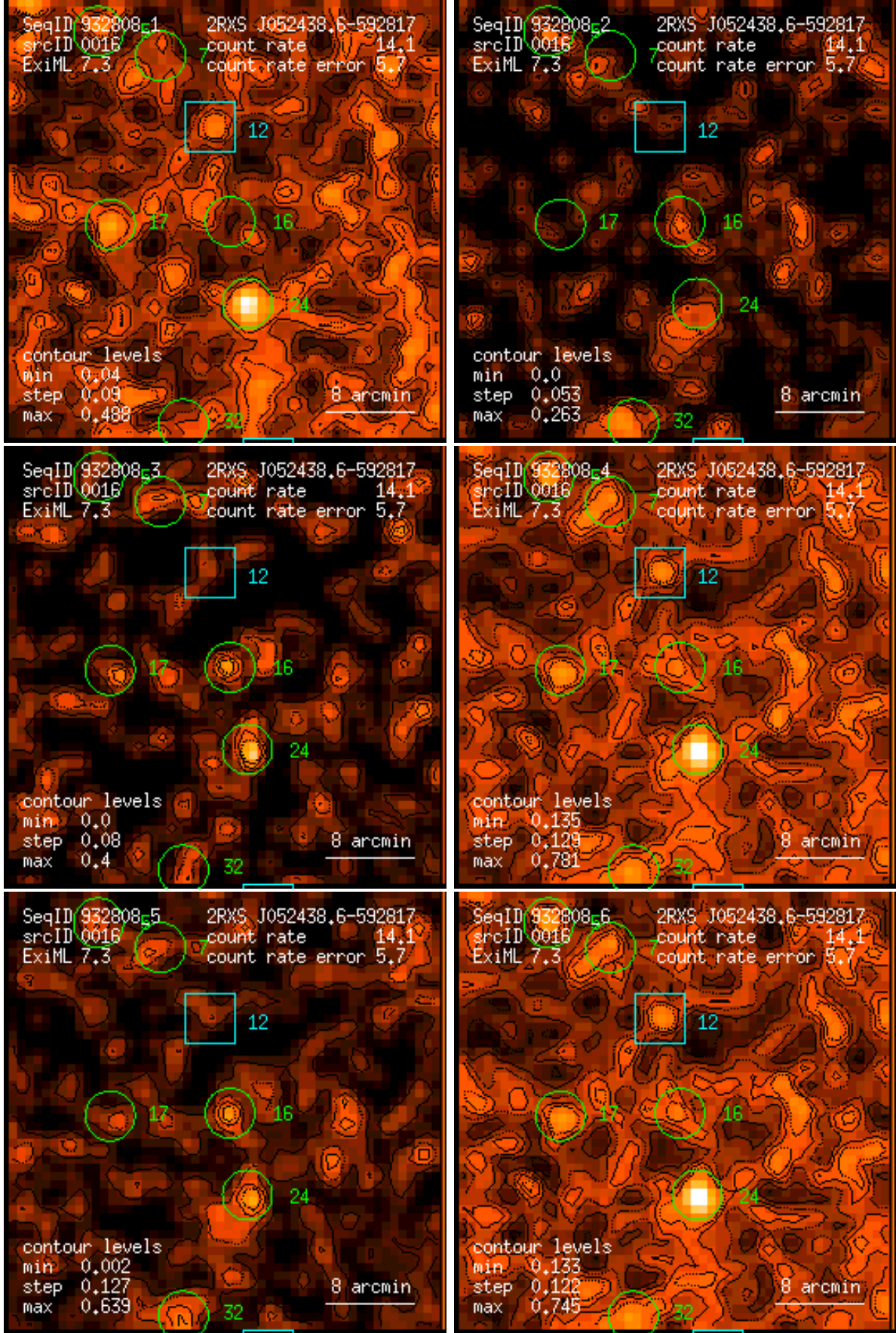
Figure 16: RASS 932808: detection 0016: band rate images, Gaussian filter: (1) PSPC channels 11 – 41, (2) 52 – 90, (3) 91 – 201, (4) 11 – 235, (5) 52 – 201, (6) 11 – 201. Broad band rates in counts/ks. Band rate contour levels in counts/ks/arcmin 2 .
