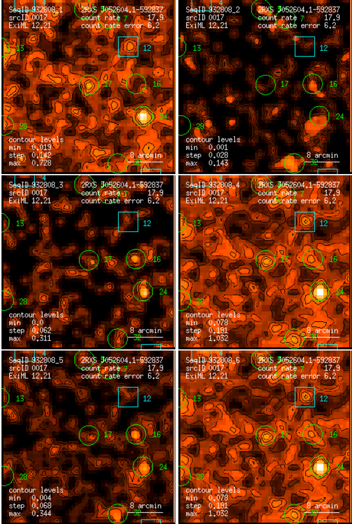
Figure 17: RASS 932808: detection 0017: band rate images, Gaussian filter: (1) PSPC channels 11 – 41, (2) 52 – 90, (3) 91 – 201, (4) 11 – 235, (5) 52 – 201, (6) 11 – 201. Broad band rates in counts/ks. Band rate contour levels in counts/ks/arcmin 2 .
