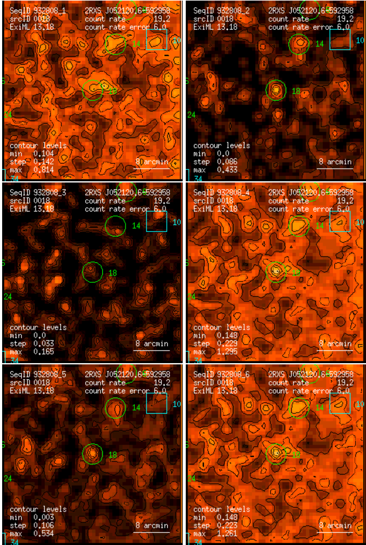
Figure 18: RASS 932808: detection 0018: band rate images, Gaussian filter: (1) PSPC channels 11 – 41, (2) 52 – 90, (3) 91 – 201, (4) 11 – 235, (5) 52 – 201, (6) 11 – 201. Broad band rates in counts/ks. Band rate contour levels in counts/ks/arcmin 2 .
