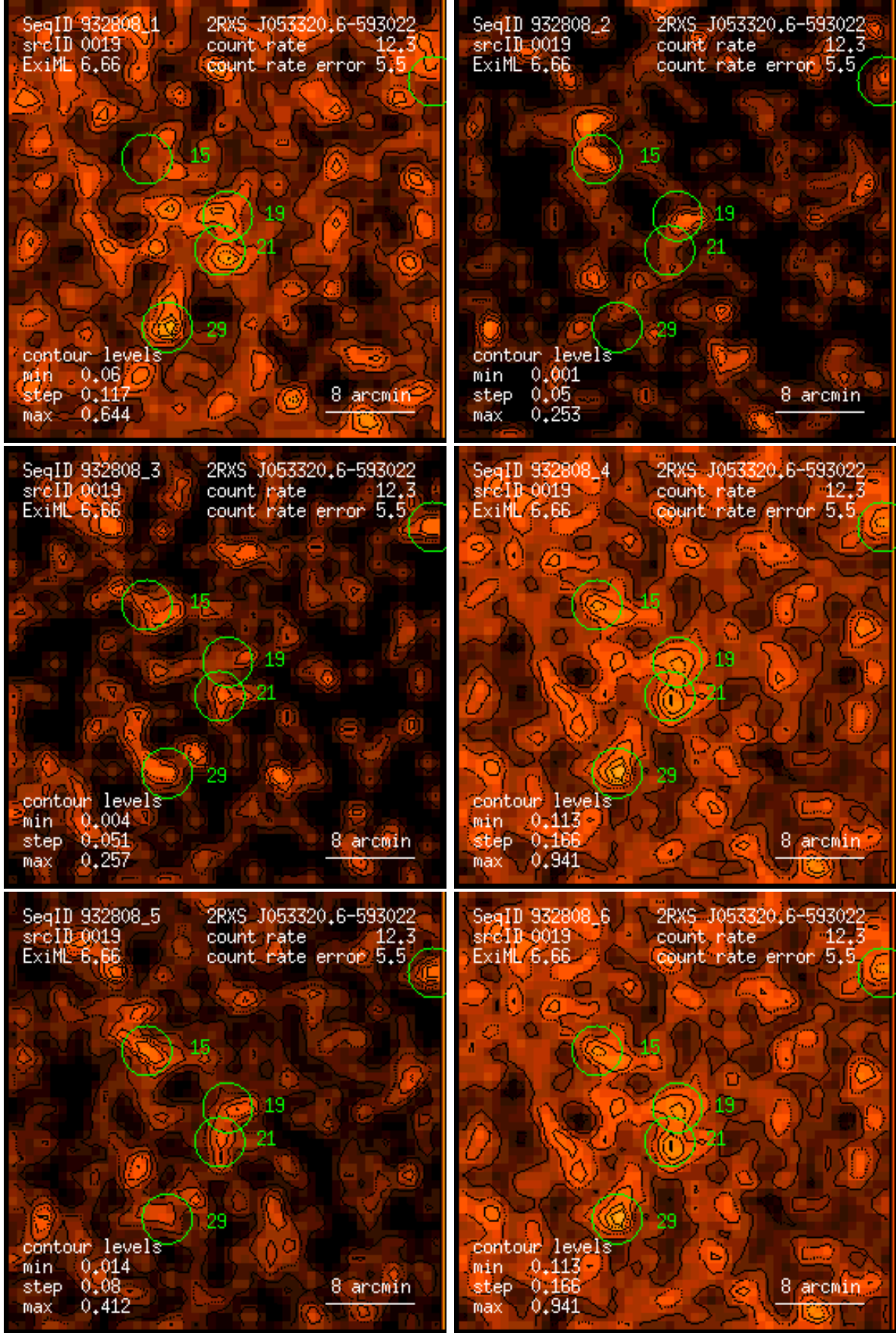
Figure 19: RASS 932808: detection 0019: band rate images, Gaussian filter: (1) PSPC channels 11 – 41, (2) 52 – 90, (3) 91 – 201, (4) 11 – 235, (5) 52 – 201, (6) 11 – 201. Broad band rates in counts/ks. Band rate contour levels in counts/ks/arcmin 2 .
