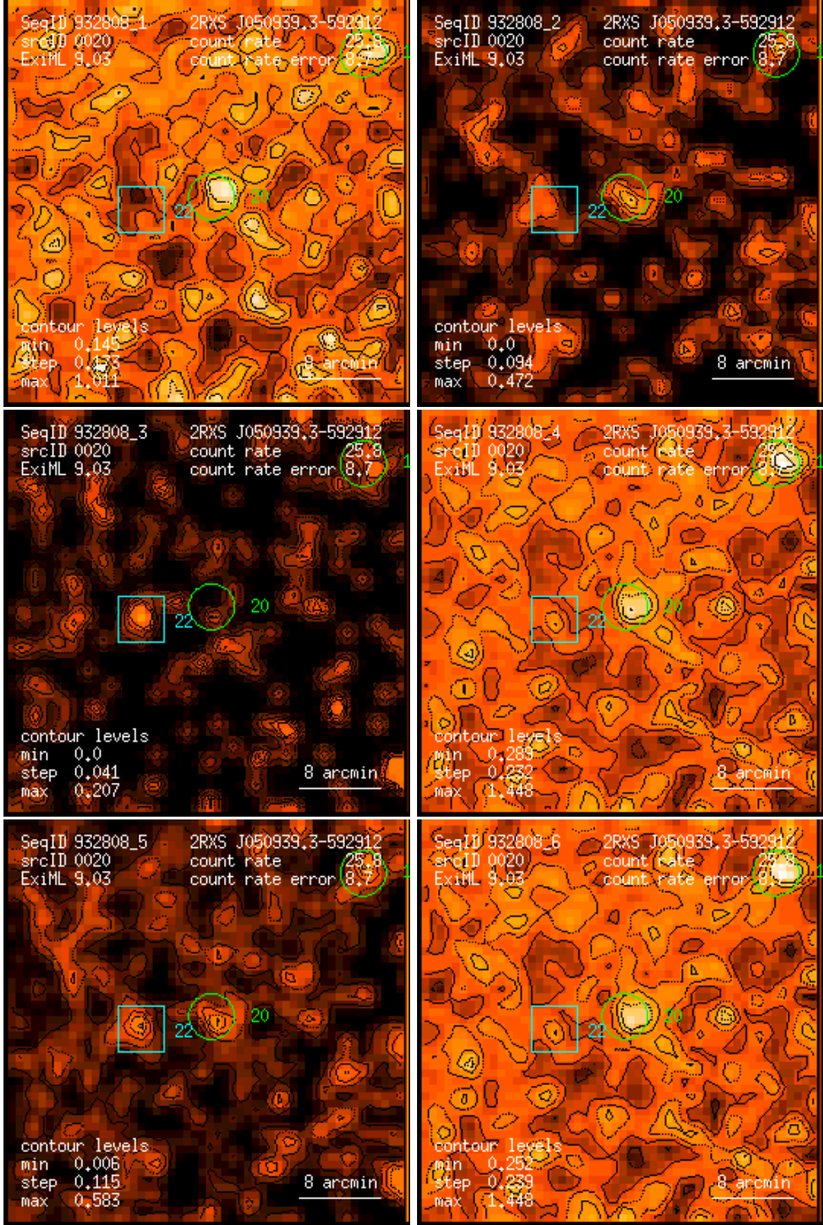
Figure 20: RASS 932808: detection 0020: band rate images, Gaussian filter: (1) PSPC channels 11 – 41, (2) 52 – 90, (3) 91 – 201, (4) 11 – 235, (5) 52 – 201, (6) 11 – 201. Broad band rates in counts/ks. Band rate contour levels in counts/ks/arcmin 2 .
