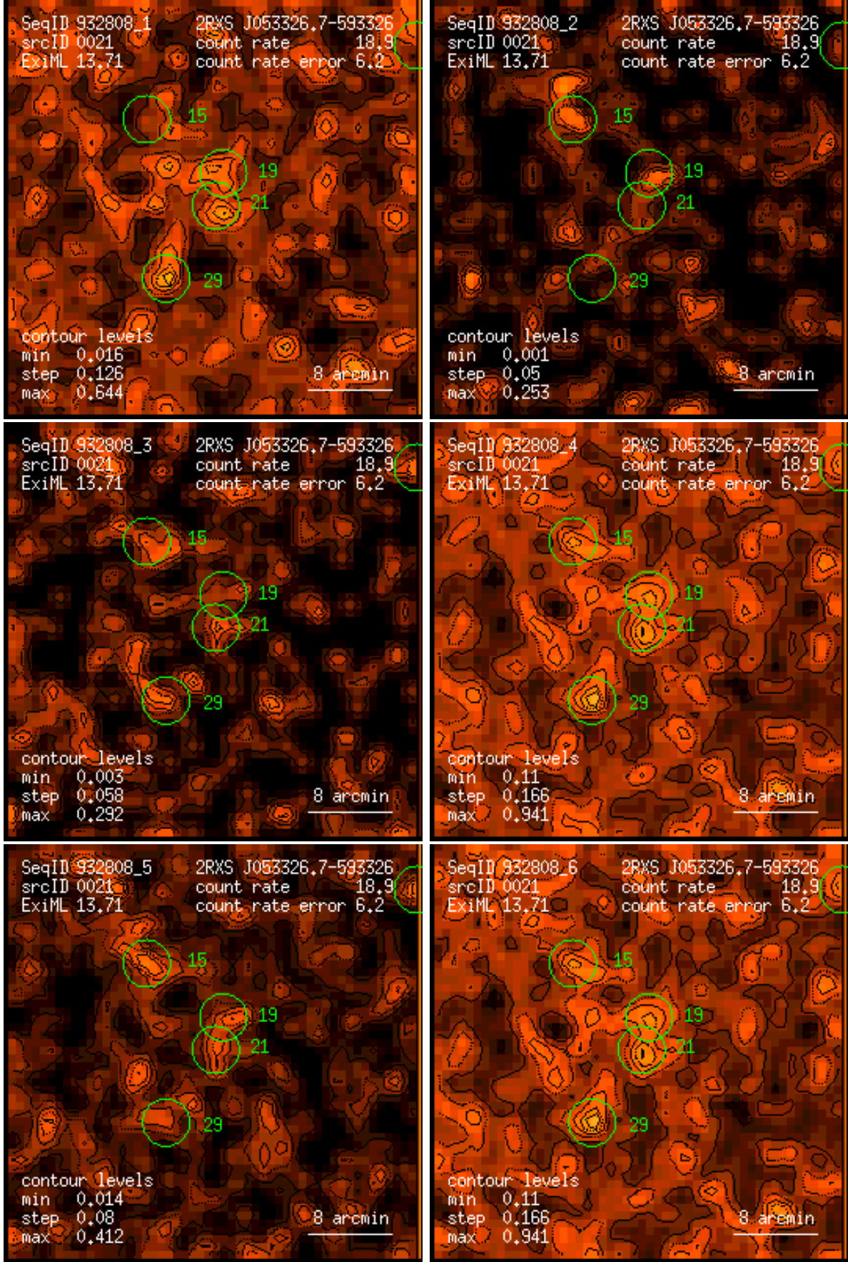
Figure 21: RASS 932808: detection 0021: band rate images, Gaussian filter: (1) PSPC channels 11 – 41, (2) 52 – 90, (3) 91 – 201, (4) 11 – 235, (5) 52 – 201, (6) 11 – 201. Broad band rates in counts/ks. Band rate contour levels in counts/ks/arcmin 2 .
