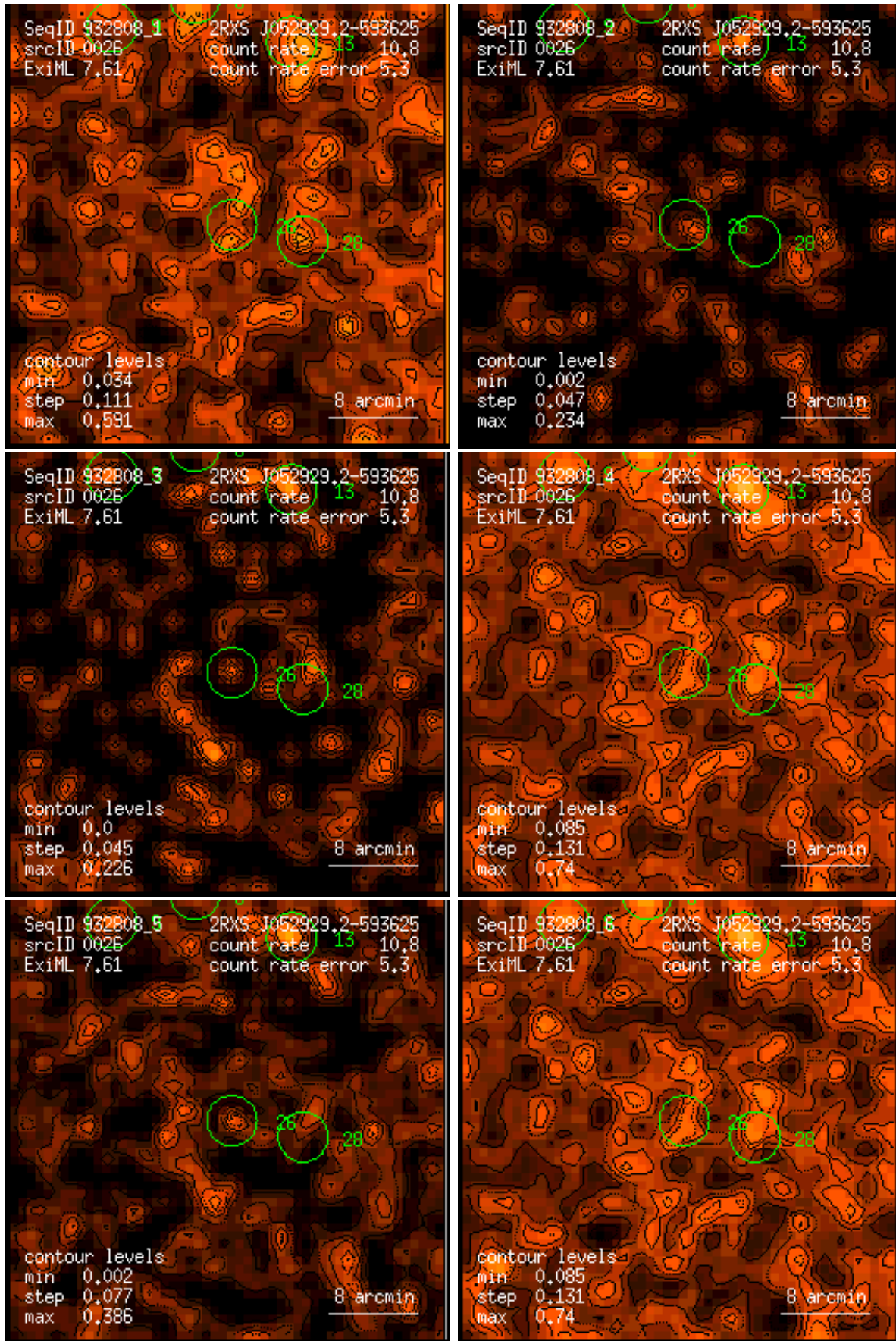
Figure 26: RASS 932808: detection 0026: band rate images, Gaussian filter: (1) PSPC channels 11 – 41, (2) 52 – 90, (3) 91 – 201, (4) 11 – 235, (5) 52 – 201, (6) 11 – 201. Broad band rates in counts/ks. Band rate contour levels in counts/ks/arcmin 2 .
