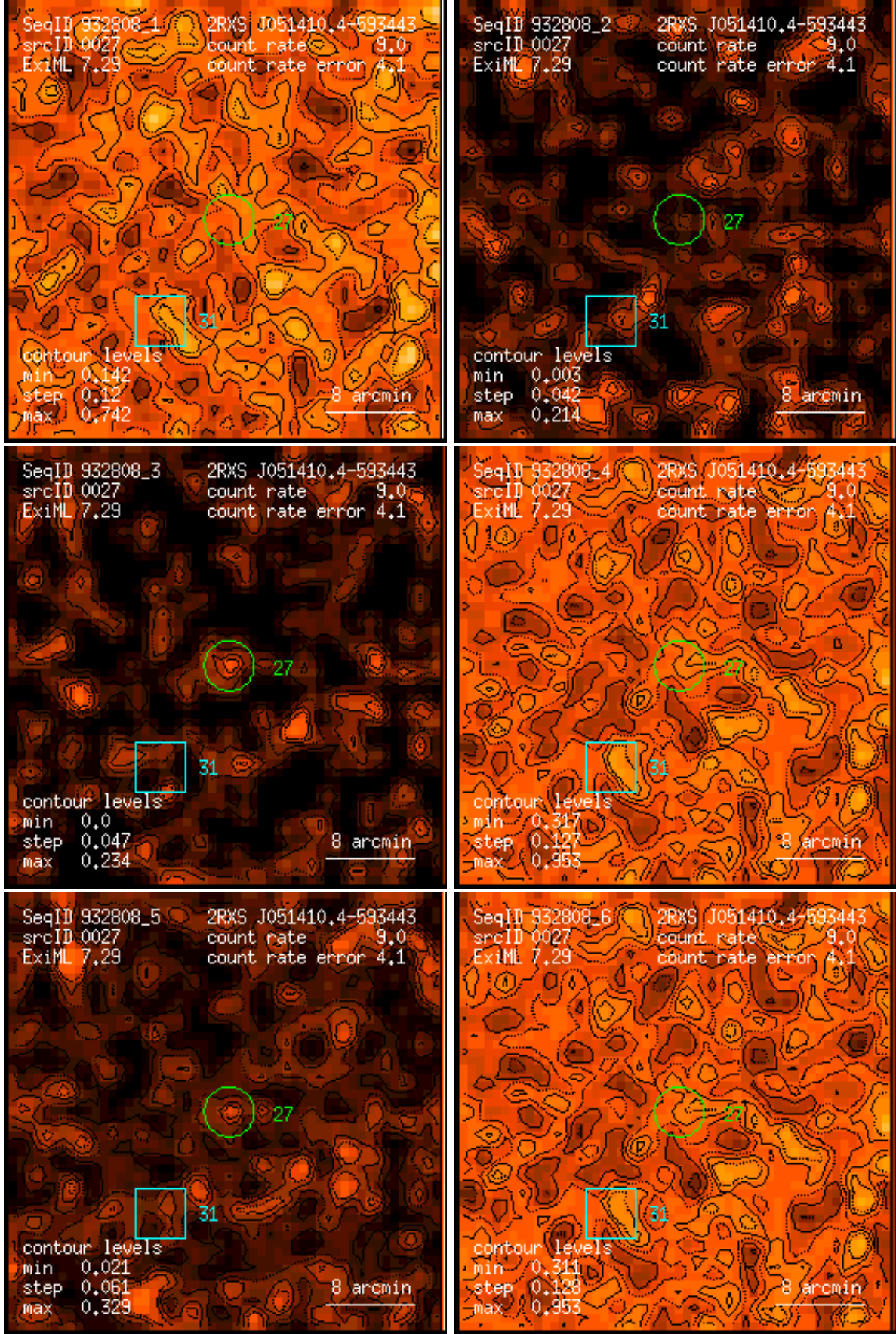
Figure 27: RASS 932808: detection 0027: band rate images, Gaussian filter: (1) PSPC channels 11 – 41, (2) 52 – 90, (3) 91 – 201, (4) 11 – 235, (5) 52 – 201, (6) 11 – 201. Broad band rates in counts/ks. Band rate contour levels in counts/ks/arcmin 2 .
