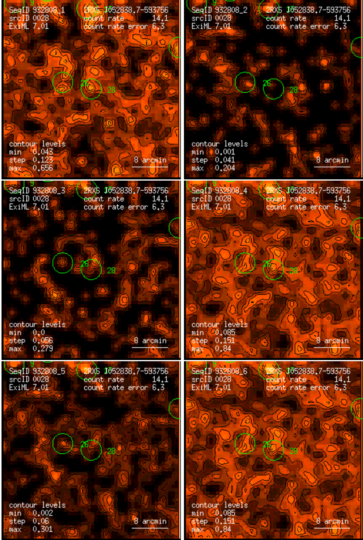
Figure 28: RASS 932808: detection 0028: band rate images, Gaussian filter: (1) PSPC channels 11 – 41, (2) 52 – 90, (3) 91 – 201, (4) 11 – 235, (5) 52 – 201, (6) 11 – 201. Broad band rates in counts/ks. Band rate contour levels in counts/ks/arcmin 2 .
