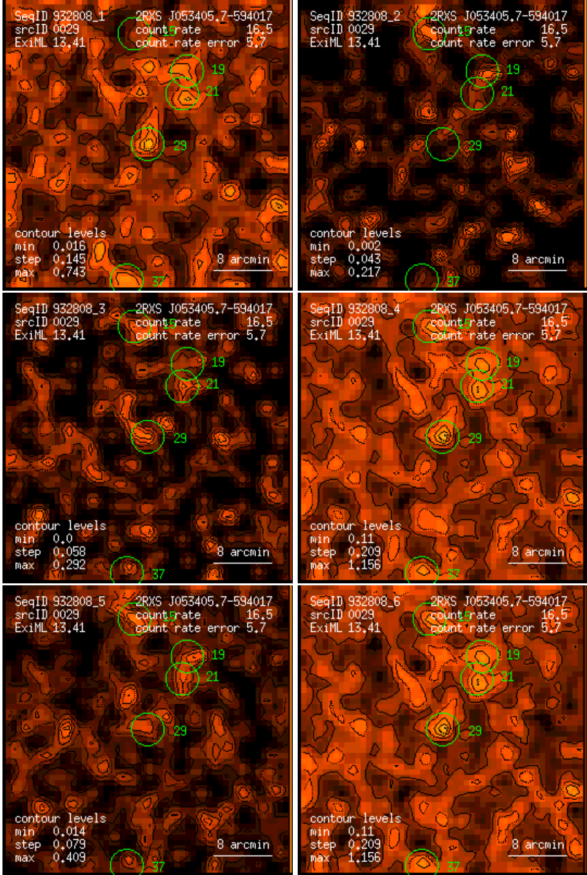
Figure 29: RASS 932808: detection 0029: band rate images, Gaussian filter: (1) PSPC channels 11 – 41, (2) 52 – 90, (3) 91 – 201, (4) 11 – 235, (5) 52 – 201, (6) 11 – 201. Broad band rates in counts/ks. Band rate contour levels in counts/ks/arcmin 2 .
