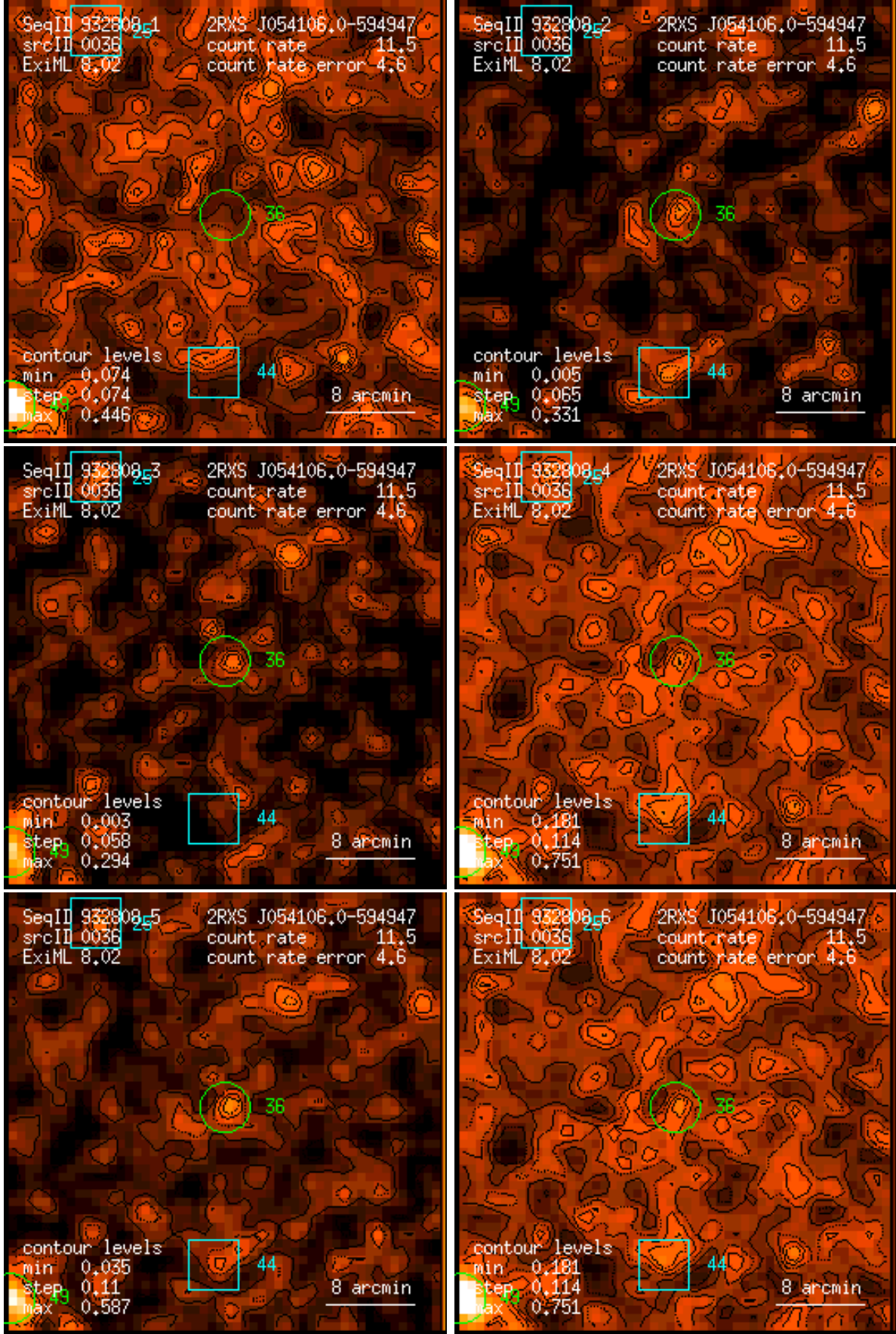
Figure 36: RASS 932808: detection 0036: band rate images, Gaussian filter: (1) PSPC channels 11 – 41, (2) 52 – 90, (3) 91 – 201, (4) 11 – 235, (5) 52 – 201, (6) 11 – 201. Broad band rates in counts/ks. Band rate contour levels in counts/ks/arcmin 2 .
