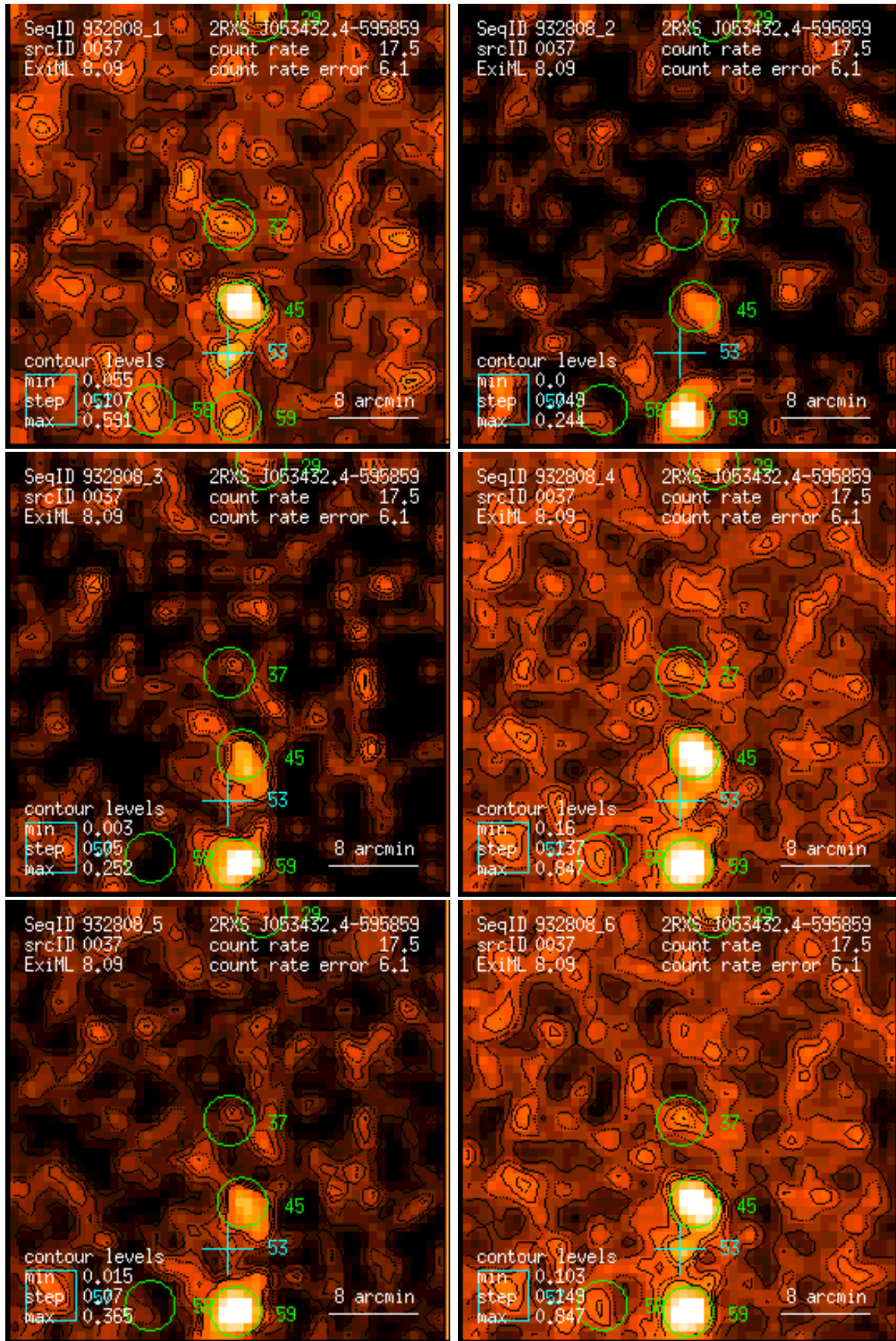
Figure 37: RASS 932808: detection 0037: band rate images, Gaussian filter: (1) PSPC channels 11 – 41, (2) 52 – 90, (3) 91 – 201, (4) 11 – 235, (5) 52 – 201, (6) 11 – 201. Broad band rates in counts/ks. Band rate contour levels in counts/ks/arcmin 2 .
