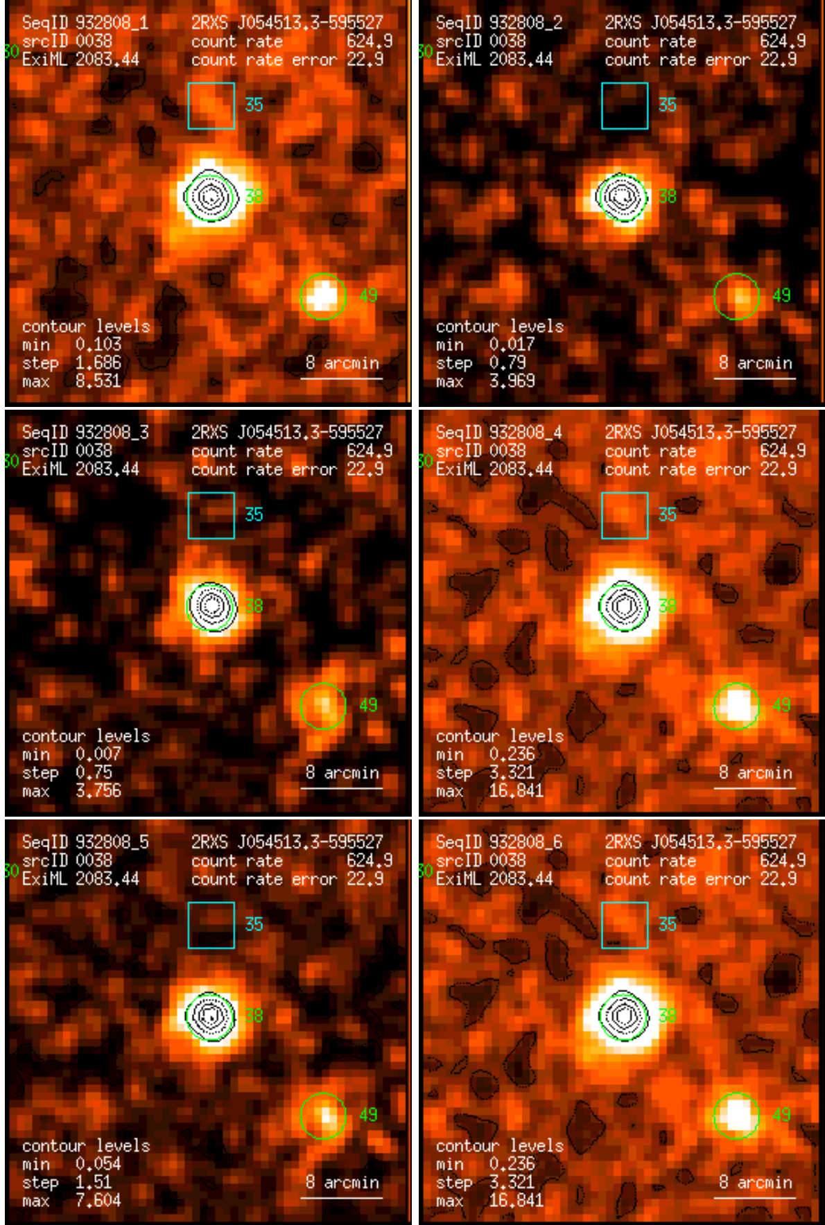
Figure 38: RASS 932808: detection 0038: band rate images, Gaussian filter: (1) PSPC channels 11 – 41, (2) 52 – 90, (3) 91 – 201, (4) 11 – 235, (5) 52 – 201, (6) 11 – 201. Broad band rates in counts/ks. Band rate contour levels in counts/ks/arcmin 2 .
