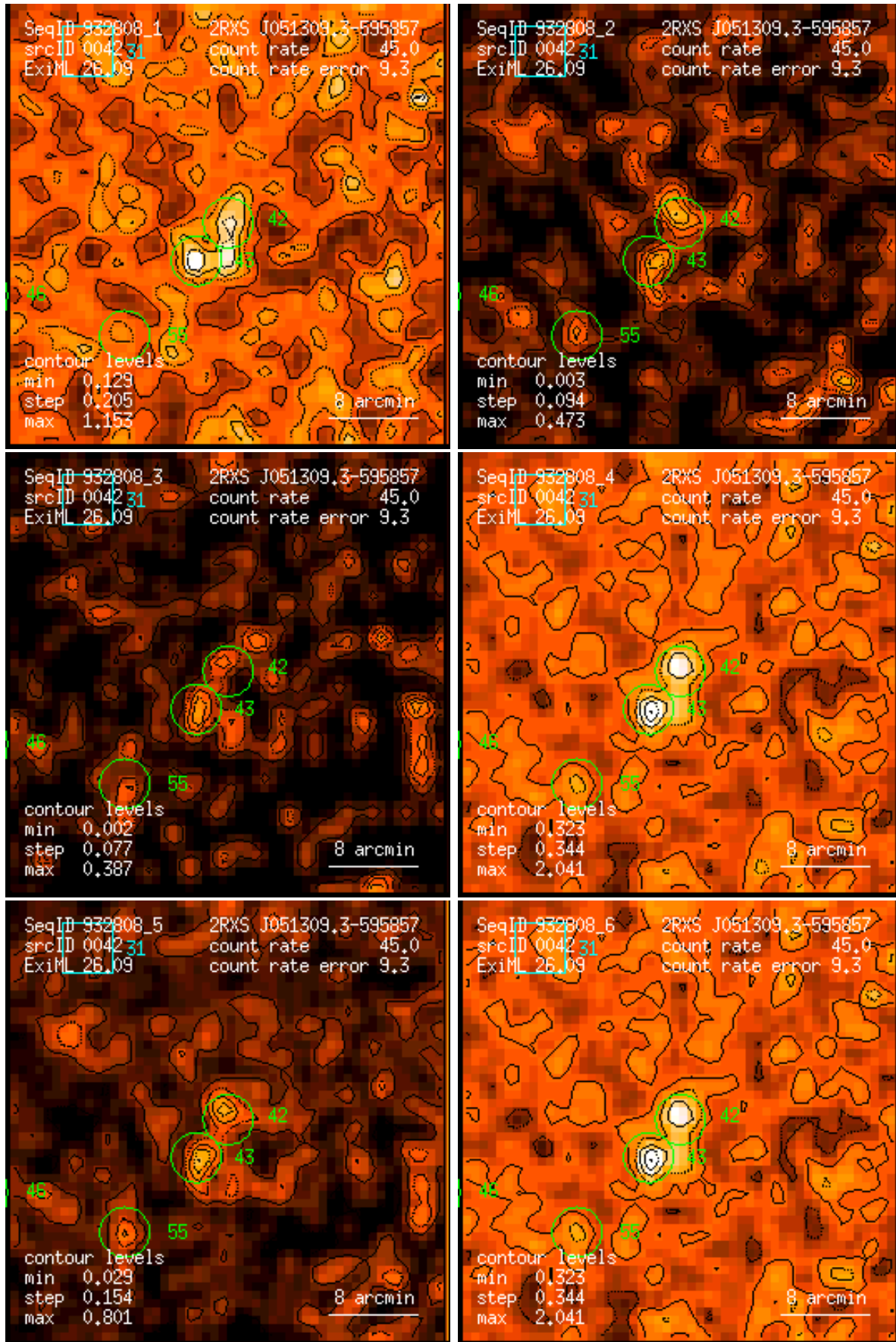
Figure 42: RASS 932808: detection 0042: band rate images, Gaussian filter: (1) PSPC channels 11 – 41, (2) 52 – 90, (3) 91 – 201, (4) 11 – 235, (5) 52 – 201, (6) 11 – 201. Broad band rates in counts/ks. Band rate contour levels in counts/ks/arcmin 2 .
