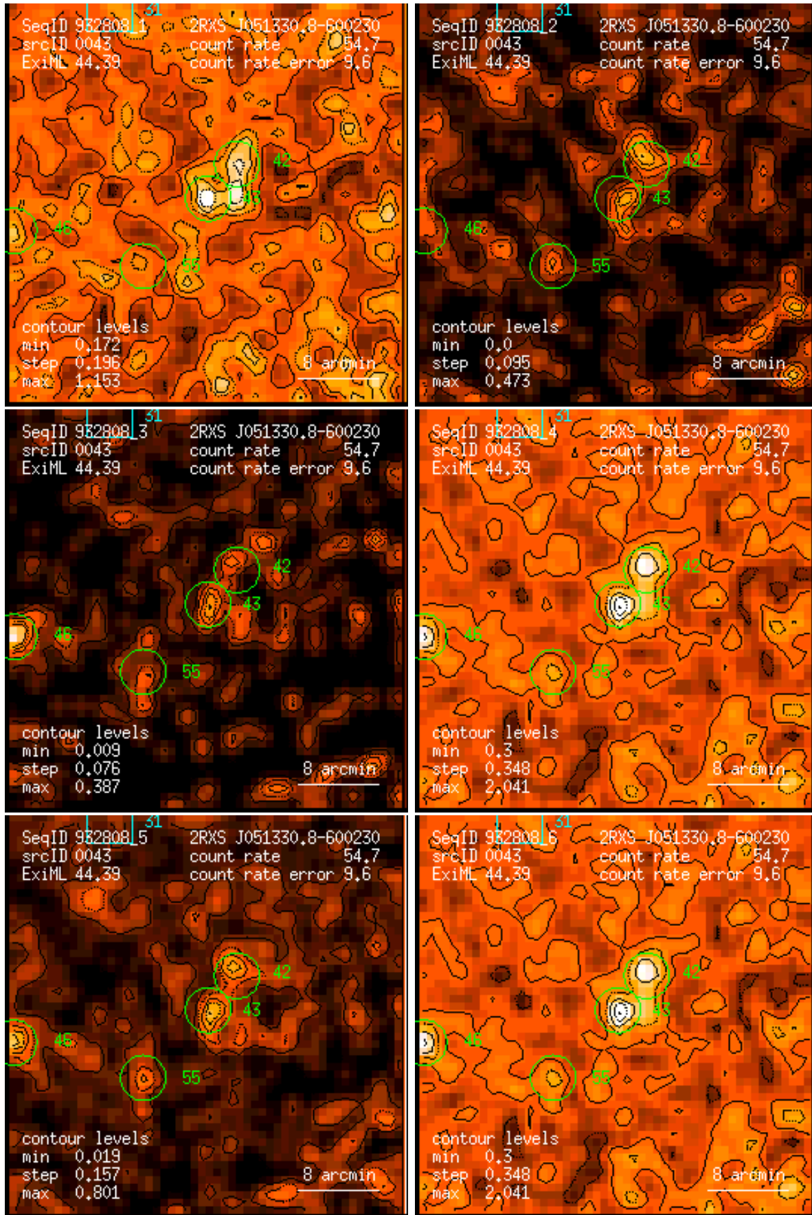
Figure 43: RASS 932808: detection 0043: band rate images, Gaussian filter: (1) PSPC channels 11 – 41, (2) 52 – 90, (3) 91 – 201, (4) 11 – 235, (5) 52 – 201, (6) 11 – 201. Broad band rates in counts/ks. Band rate contour levels in counts/ks/arcmin 2 .
