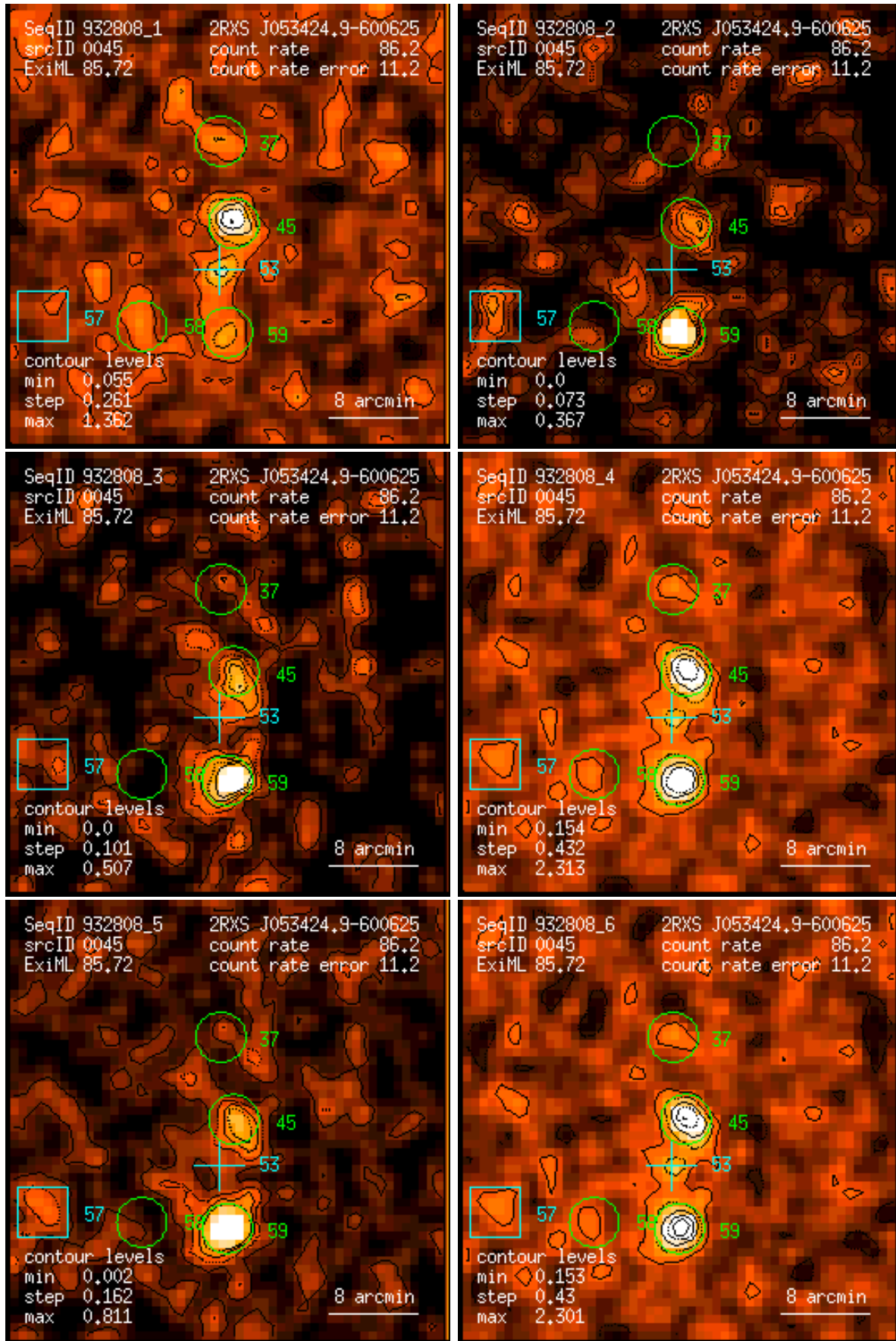
Figure 45: RASS 932808: detection 0045: band rate images, Gaussian filter: (1) PSPC channels 11 – 41, (2) 52 – 90, (3) 91 – 201, (4) 11 – 235, (5) 52 – 201, (6) 11 – 201. Broad band rates in counts/ks. Band rate contour levels in counts/ks/arcmin 2 .
