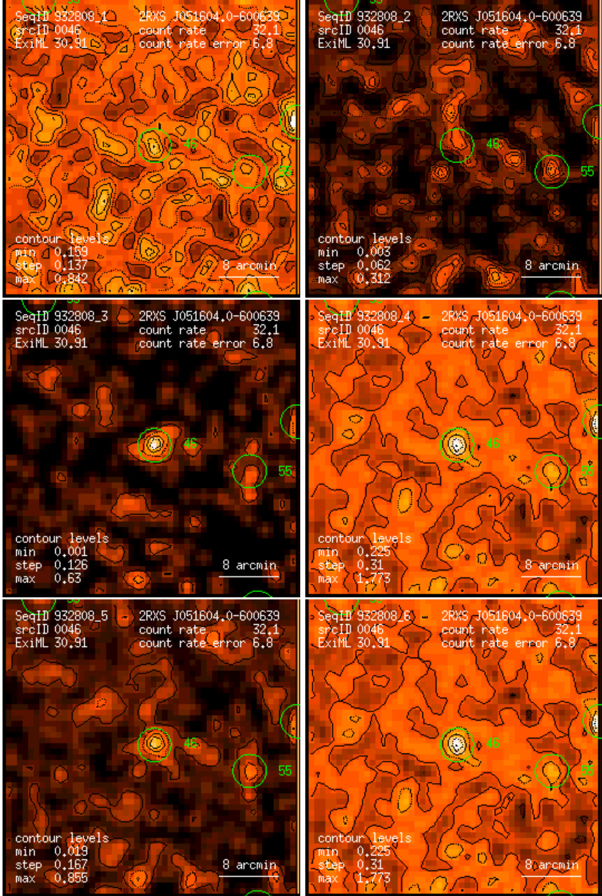
Figure 46: RASS 932808: detection 0046: band rate images, Gaussian filter: (1) PSPC channels 11 – 41, (2) 52 – 90, (3) 91 – 201, (4) 11 – 235, (5) 52 – 201, (6) 11 – 201. Broad band rates in counts/ks. Band rate contour levels in counts/ks/arcmin 2 .
