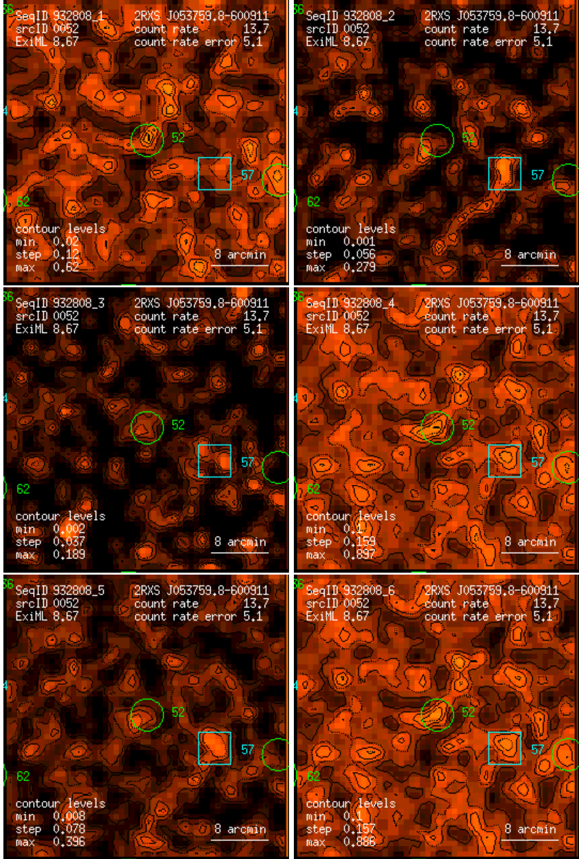
Figure 52: RASS 932808: detection 0052: band rate images, Gaussian filter: (1) PSPC channels 11 – 41, (2) 52 – 90, (3) 91 – 201, (4) 11 – 235, (5) 52 – 201, (6) 11 – 201. Broad band rates in counts/ks. Band rate contour levels in counts/ks/arcmin 2 .
