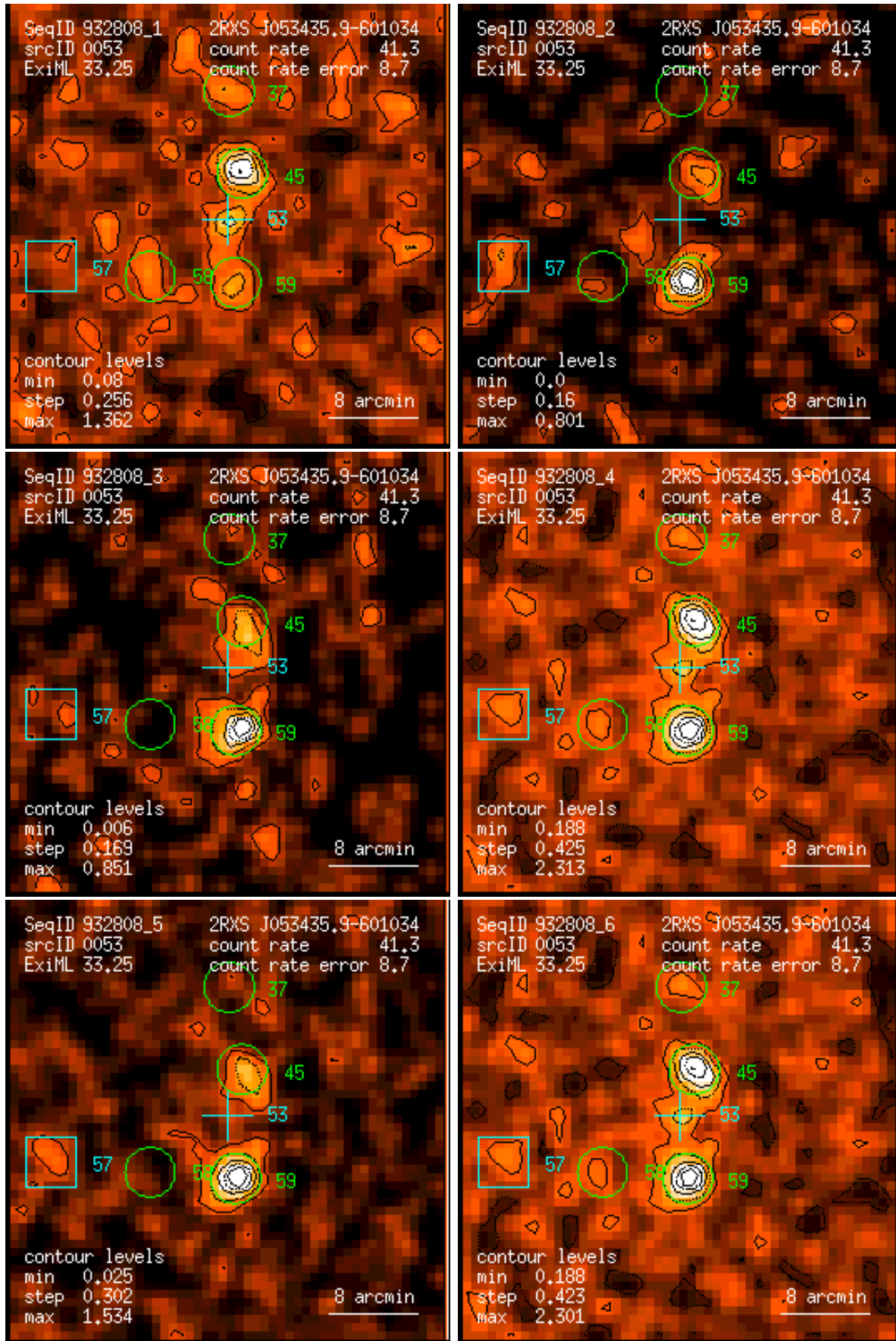
Figure 53: RASS 932808: detection 0053: band rate images, Gaussian filter: (1) PSPC channels 11 – 41, (2) 52 – 90, (3) 91 – 201, (4) 11 – 235, (5) 52 – 201, (6) 11 – 201. Broad band rates in counts/ks. Band rate contour levels in counts/ks/arcmin 2 .
