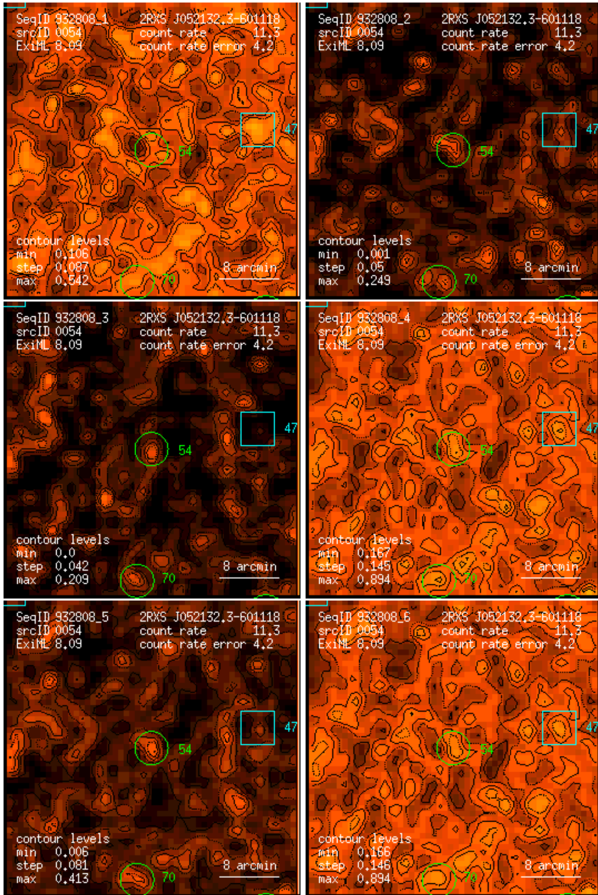
Figure 54: RASS 932808: detection 0054: band rate images, Gaussian filter: (1) PSPC channels 11 – 41, (2) 52 – 90, (3) 91 – 201, (4) 11 – 235, (5) 52 – 201, (6) 11 – 201. Broad band rates in counts/ks. Band rate contour levels in counts/ks/arcmin 2 .
