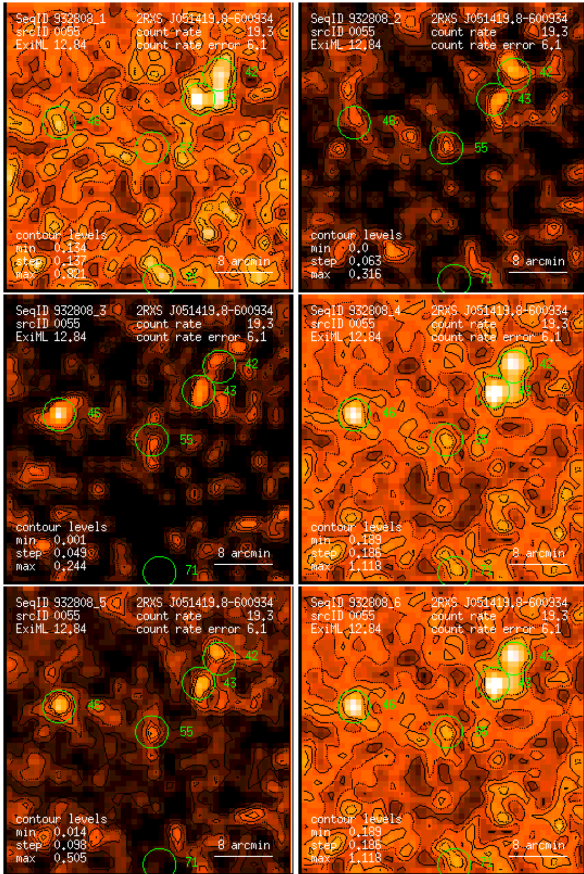
Figure 55: RASS 932808: detection 0055: band rate images, Gaussian filter: (1) PSPC channels 11 – 41, (2) 52 – 90, (3) 91 – 201, (4) 11 – 235, (5) 52 – 201, (6) 11 – 201. Broad band rates in counts/ks. Band rate contour levels in counts/ks/arcmin 2 .
