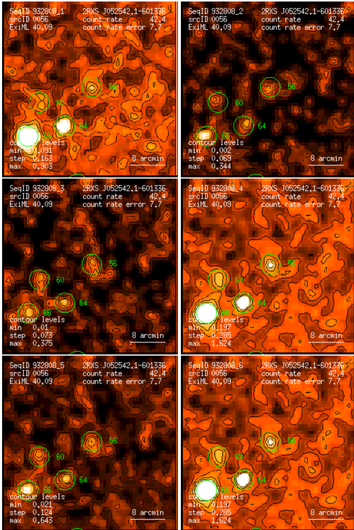
Figure 56: RASS 932808: detection 0056: band rate images, Gaussian filter: (1) PSPC channels 11 – 41, (2) 52 – 90, (3) 91 – 201, (4) 11 – 235, (5) 52 – 201, (6) 11 – 201. Broad band rates in counts/ks. Band rate contour levels in counts/ks/arcmin 2 .
