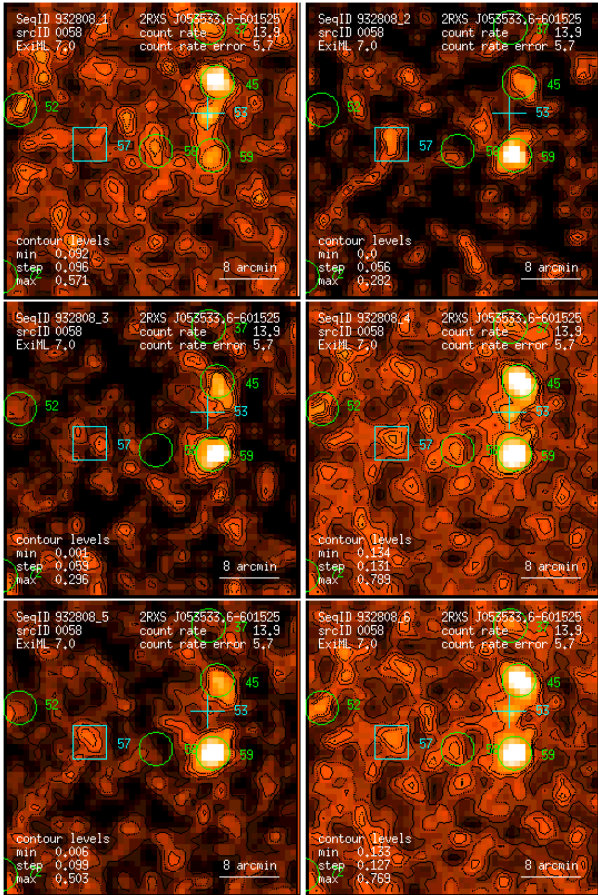
Figure 58: RASS 932808: detection 0058: band rate images, Gaussian filter: (1) PSPC channels 11 – 41, (2) 52 – 90, (3) 91 – 201, (4) 11 – 235, (5) 52 – 201, (6) 11 – 201. Broad band rates in counts/ks. Band rate contour levels in counts/ks/arcmin 2 .
