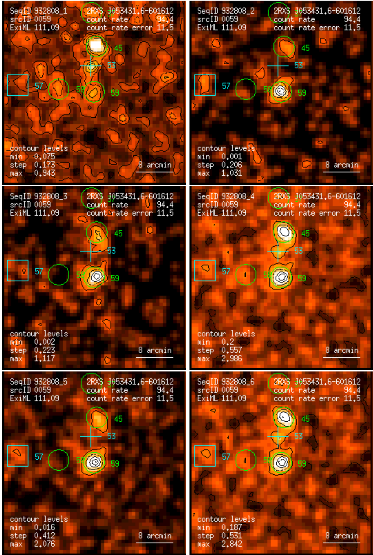
Figure 59: RASS 932808: detection 0059: band rate images, Gaussian filter: (1) PSPC channels 11 – 41, (2) 52 – 90, (3) 91 – 201, (4) 11 – 235, (5) 52 – 201, (6) 11 – 201. Broad band rates in counts/ks. Band rate contour levels in counts/ks/arcmin 2 .
