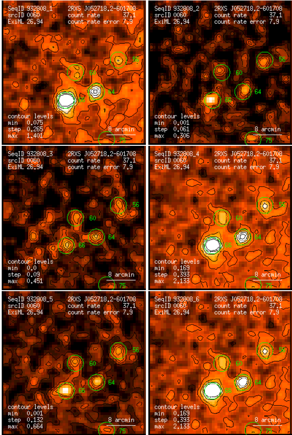
Figure 60: RASS 932808: detection 0060: band rate images, Gaussian filter: (1) PSPC channels 11 – 41, (2) 52 – 90, (3) 91 – 201, (4) 11 – 235, (5) 52 – 201, (6) 11 – 201. Broad band rates in counts/ks. Band rate contour levels in counts/ks/arcmin 2 .
