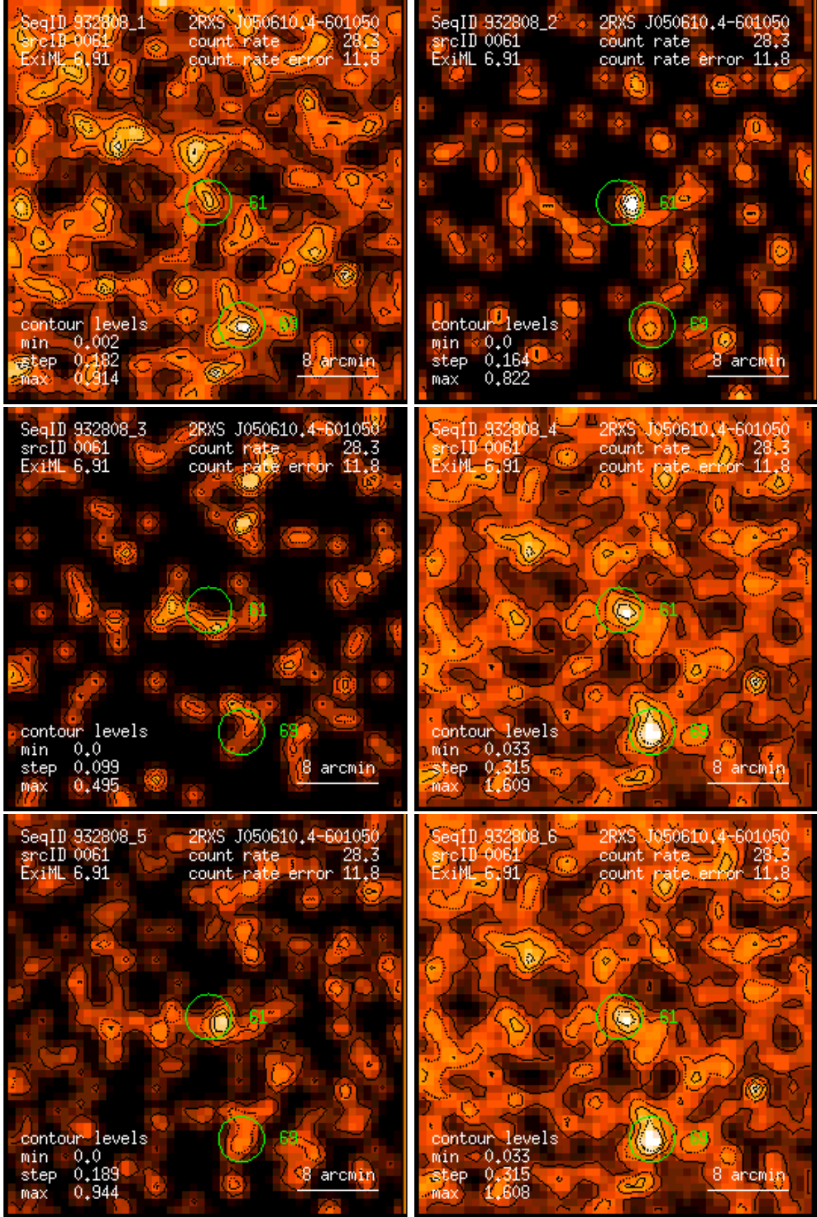
Figure 61: RASS 932808: detection 0061: band rate images, Gaussian filter: (1) PSPC channels 11 – 41, (2) 52 – 90, (3) 91 – 201, (4) 11 – 235, (5) 52 – 201, (6) 11 – 201. Broad band rates in counts/ks. Band rate contour levels in counts/ks/arcmin 2 .
