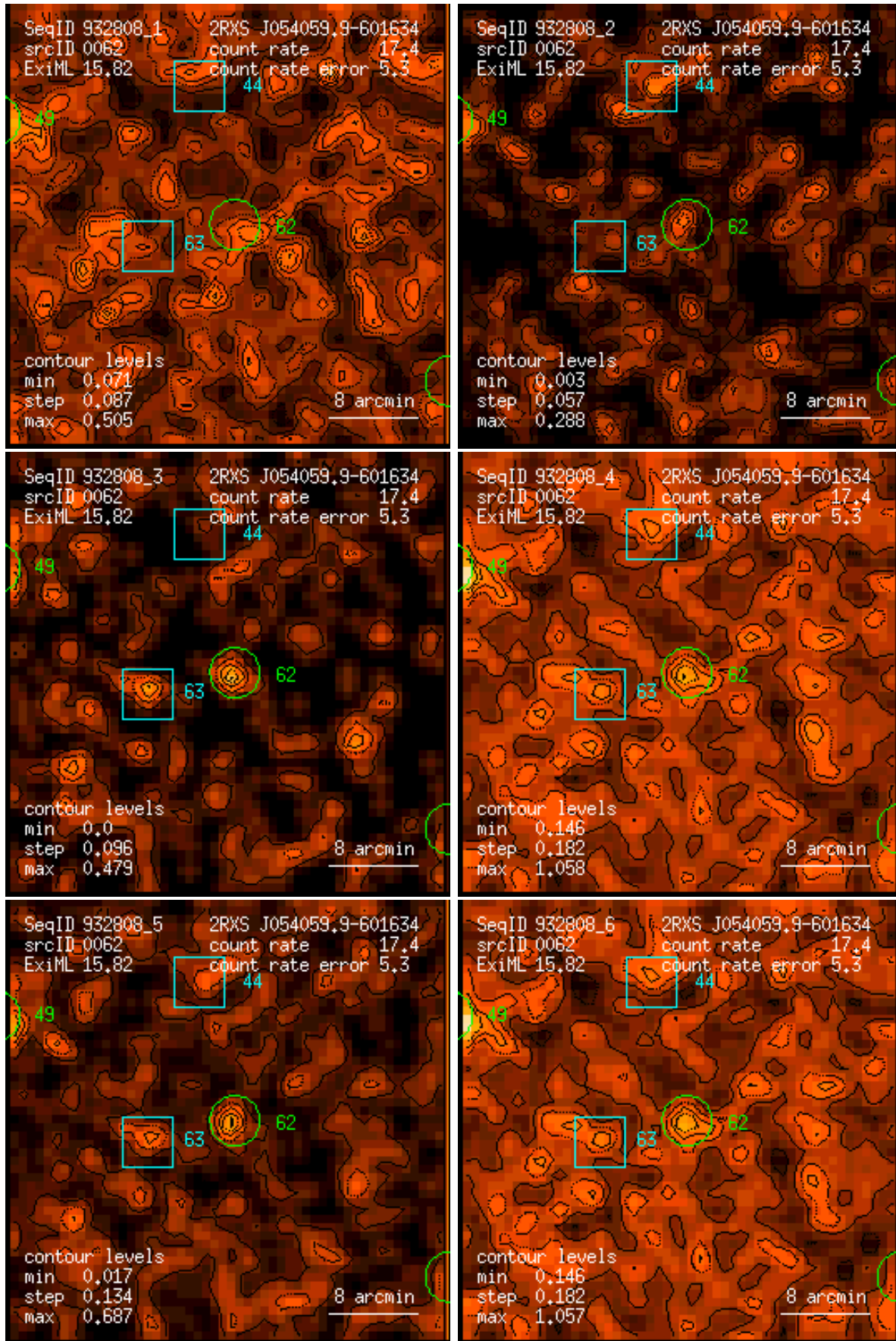
Figure 62: RASS 932808: detection 0062: band rate images, Gaussian filter: (1) PSPC channels 11 – 41, (2) 52 – 90, (3) 91 – 201, (4) 11 – 235, (5) 52 – 201, (6) 11 – 201. Broad band rates in counts/ks. Band rate contour levels in counts/ks/arcmin 2 .
