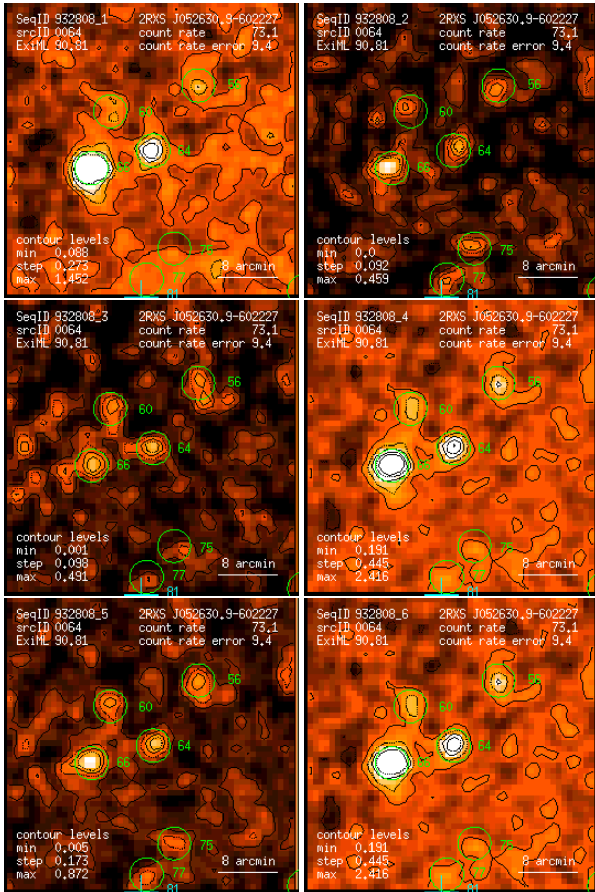
Figure 64: RASS 932808: detection 0064: band rate images, Gaussian filter: (1) PSPC channels 11 – 41, (2) 52 – 90, (3) 91 – 201, (4) 11 – 235, (5) 52 – 201, (6) 11 – 201. Broad band rates in counts/ks. Band rate contour levels in counts/ks/arcmin 2 .
