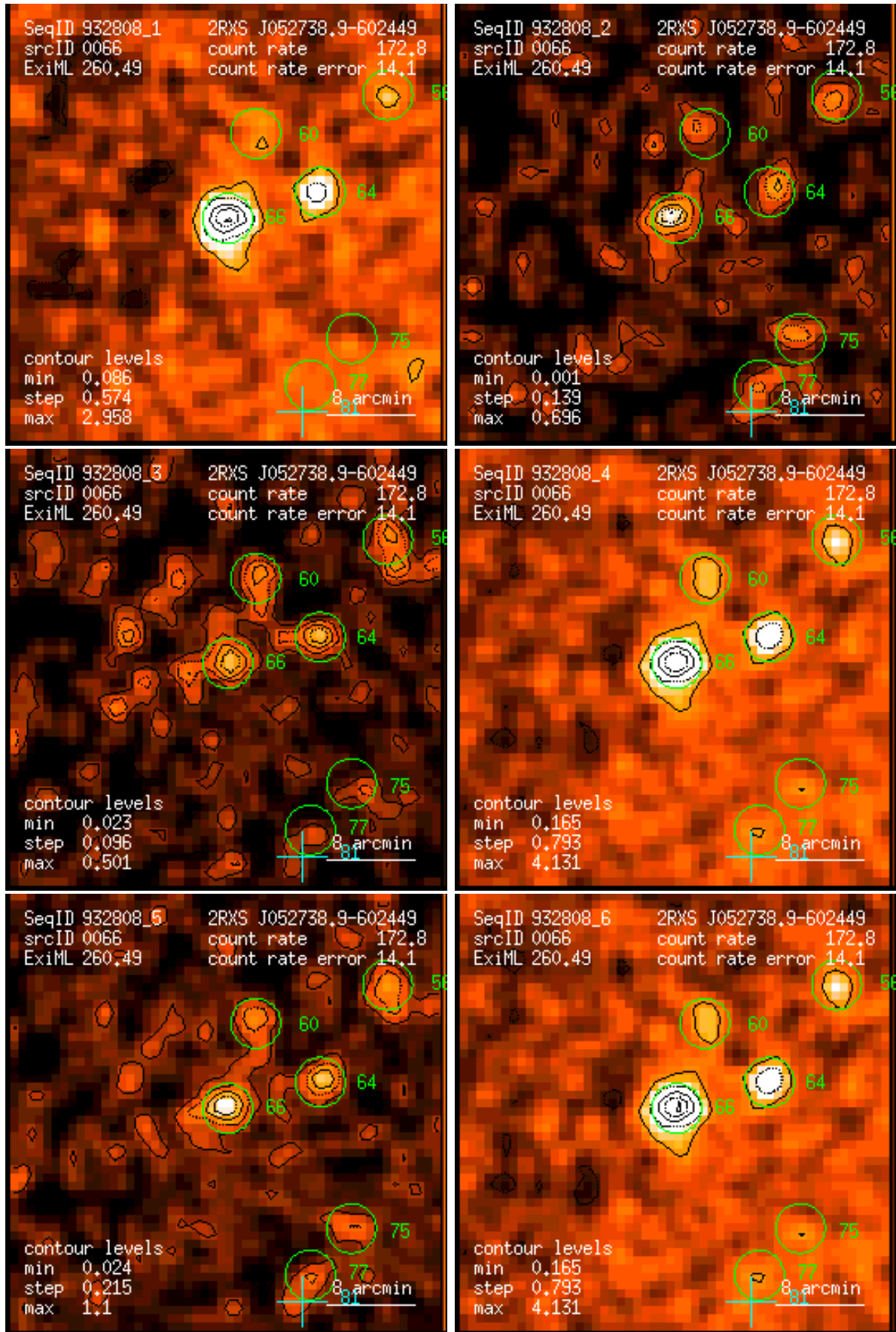
Figure 66: RASS 932808: detection 0066: band rate images, Gaussian filter: (1) PSPC channels 11 – 41, (2) 52 – 90, (3) 91 – 201, (4) 11 – 235, (5) 52 – 201, (6) 11 – 201. Broad band rates in counts/ks. Band rate contour levels in counts/ks/arcmin 2 .
