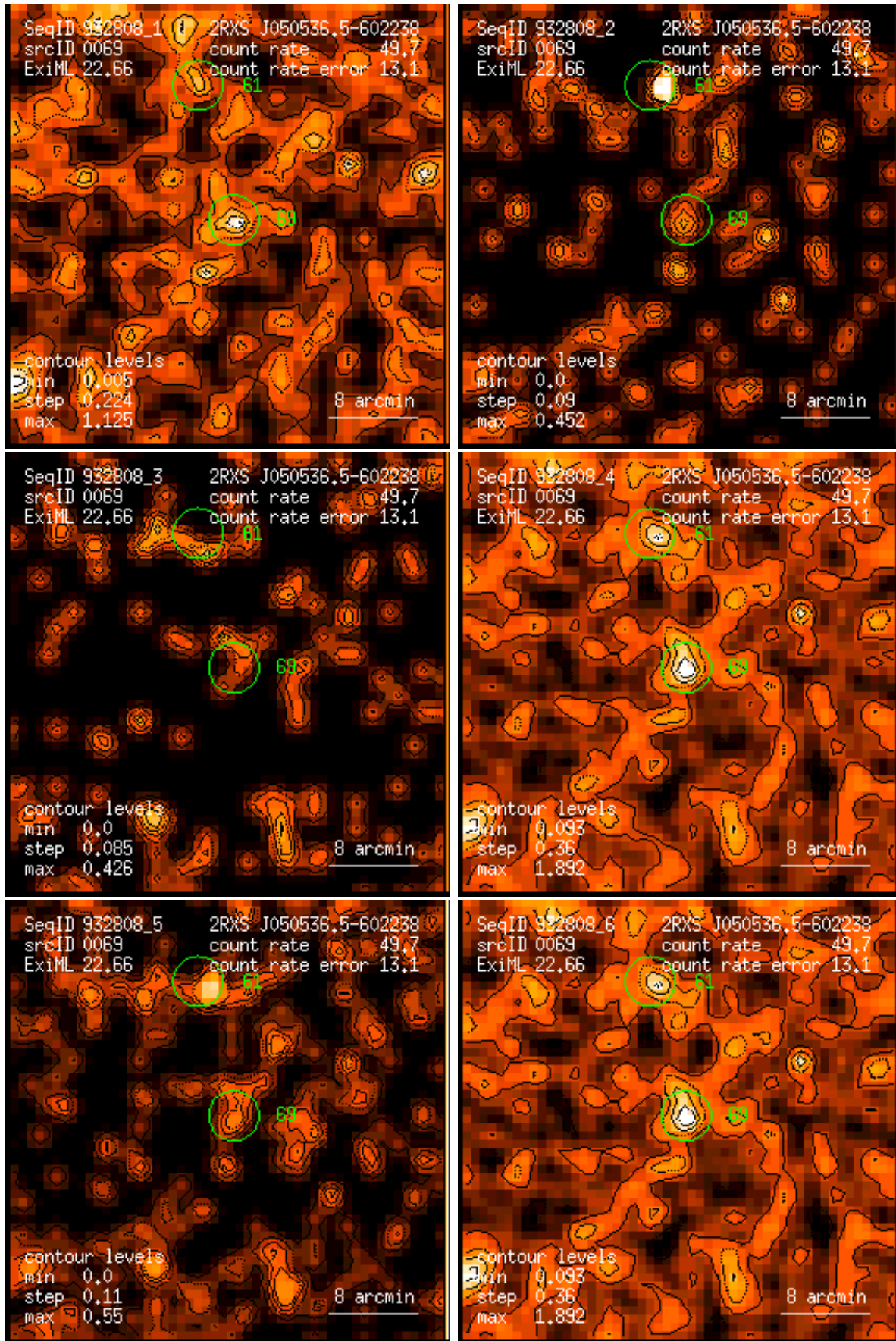
Figure 69: RASS 932808: detection 0069: band rate images, Gaussian filter: (1) PSPC channels 11 – 41, (2) 52 – 90, (3) 91 – 201, (4) 11 – 235, (5) 52 – 201, (6) 11 – 201. Broad band rates in counts/ks. Band rate contour levels in counts/ks/arcmin 2 .
