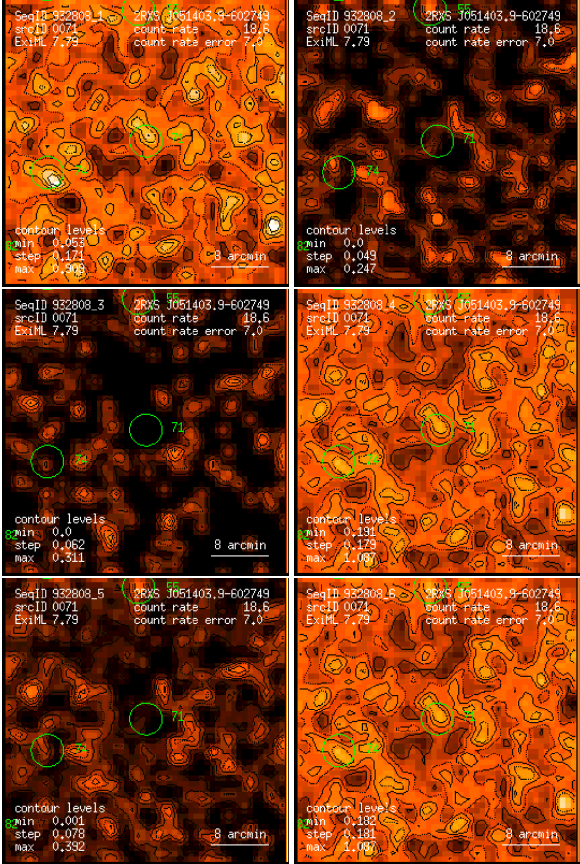
Figure 71: RASS 932808: detection 0071: band rate images, Gaussian filter: (1) PSPC channels 11 – 41, (2) 52 – 90, (3) 91 – 201, (4) 11 – 235, (5) 52 – 201, (6) 11 – 201. Broad band rates in counts/ks. Band rate contour levels in counts/ks/arcmin 2 .
